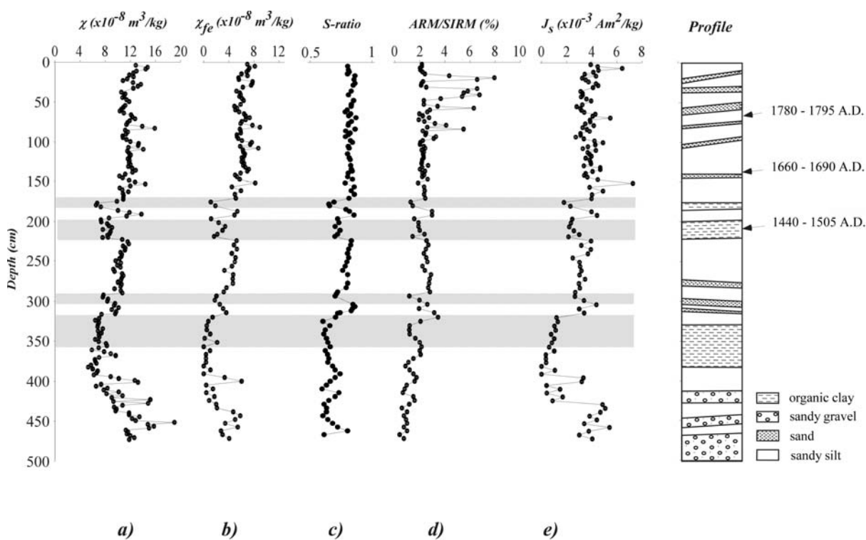
Fig. 3-3 Mineral magnetic parameters measured throughout the sedimentary profile in Spirálka Cave – a) magnetic susceptibility, b) ferromagnetic susceptibility, c) S-ratio (see text), d) ratio of anhysteretic remanent magnetization and saturation isothermal magnetization and e) saturation magnetization. Highlighted are the zones with anomalously low magnetic susceptibility (see text). Also shown is a sketch of the sampled profile showing position of the radiocarbon dated charcoal and wood samples.
