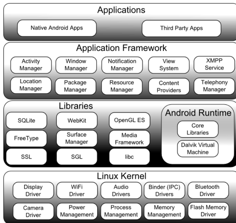
Figure 2: Main Components/Architecture of Android Platform.
