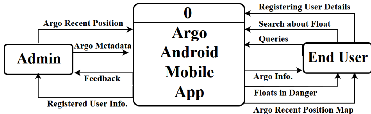
Figure 4: Context Diagram of Argo Android App.
