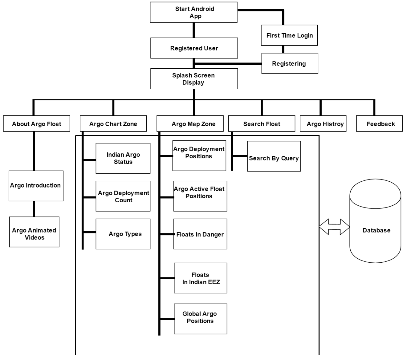
Figure 5: Architecture of Argo Android App
