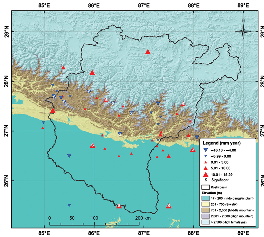
Figure 13. Trends in annual total PRCP when RR > 95th percentile (R95p).
