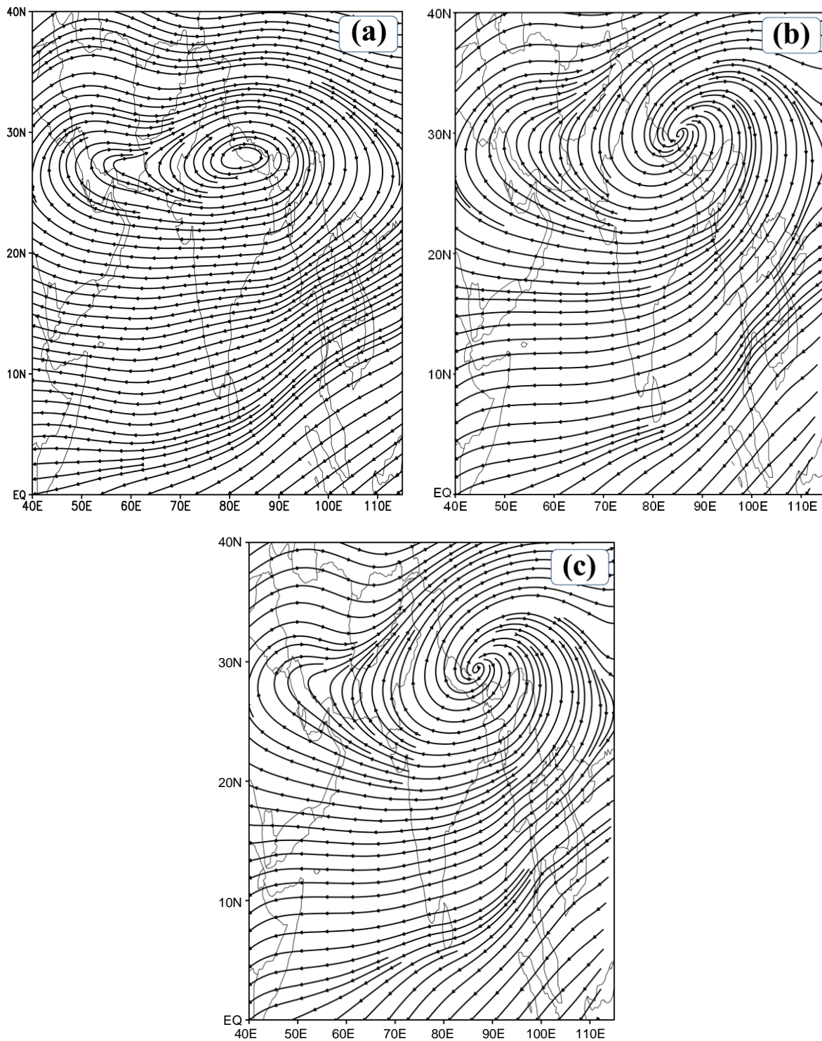
Figure 7. Same as Figure 5 but for streamlines at 200 hPa signifying the TA.
