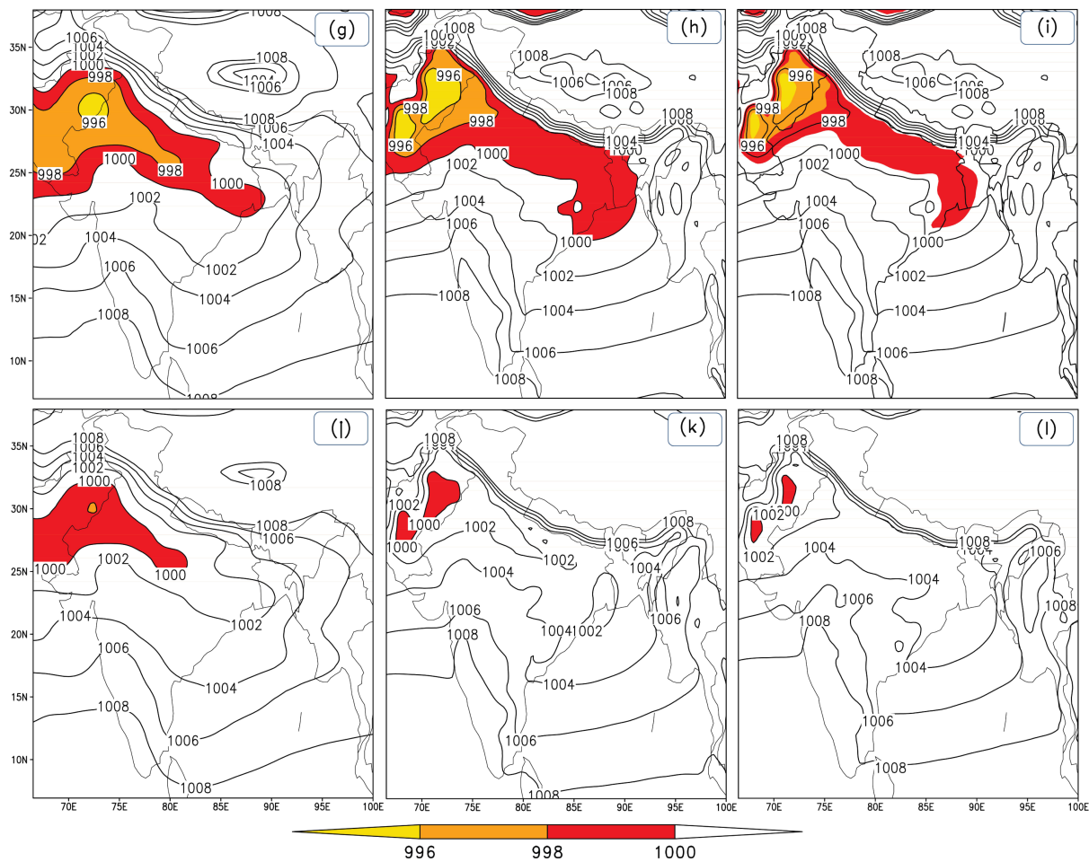
Figure 3. Composite mean sea level pressure (hPa) for the months May, June, July and the season June-September for observed ((a), (d), (g), (j)); historical simulations ((b), (e), (h), (k)) based on 1951-2000 and mean sea level pressure under RCP4.5 ((c), (f), (i), (l)) based on 2051-2100 depicting the heat low over north west India.
