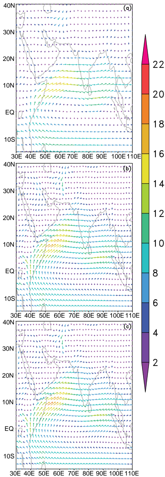
Figure 5. Mean 850 hPa vector winds (m/s) for June through September signifying the LLJ for (a) Observed, (b) historical based on 1951-2000 and (c) Under RCP4.5 based on 2051-2100.
