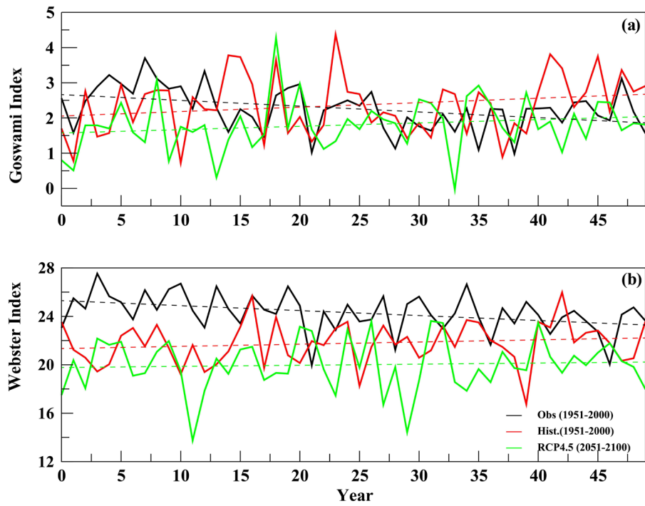
Figure 2. Time series of (a) Goswami Wind Index and (b) Webster Yang Index for observed, historical and RCP4.5 simulations.
