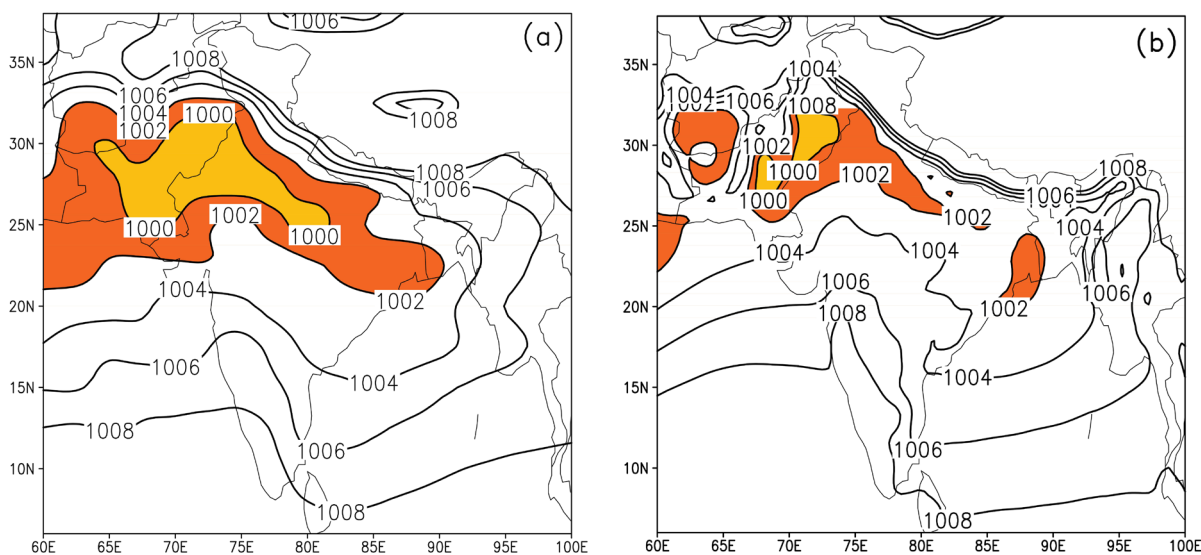
Figure 3. Composite mean sea level pressure (hPa) for the months May, June, July and the season June-September for observed ((a), (d), (g), (j)); historical simulations ((b), (e), (h), (k)) based on 1951-2000 and mean sea level pressure under RCP4.5 ((c), (f), (i), (l)) based on 2051-2100 depicting the heat low over north west India.
