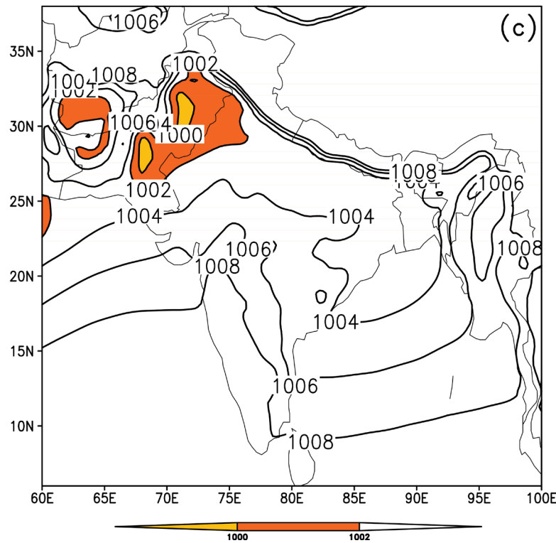
Figure 4. Composite June to September mean Sea level pressure (hPa) pattern based on 1951-2000 over monsoon trough region (a) Observed, (b) Historical for 1951-2000 and (c) RCP4.5 based on 2051-2100.
