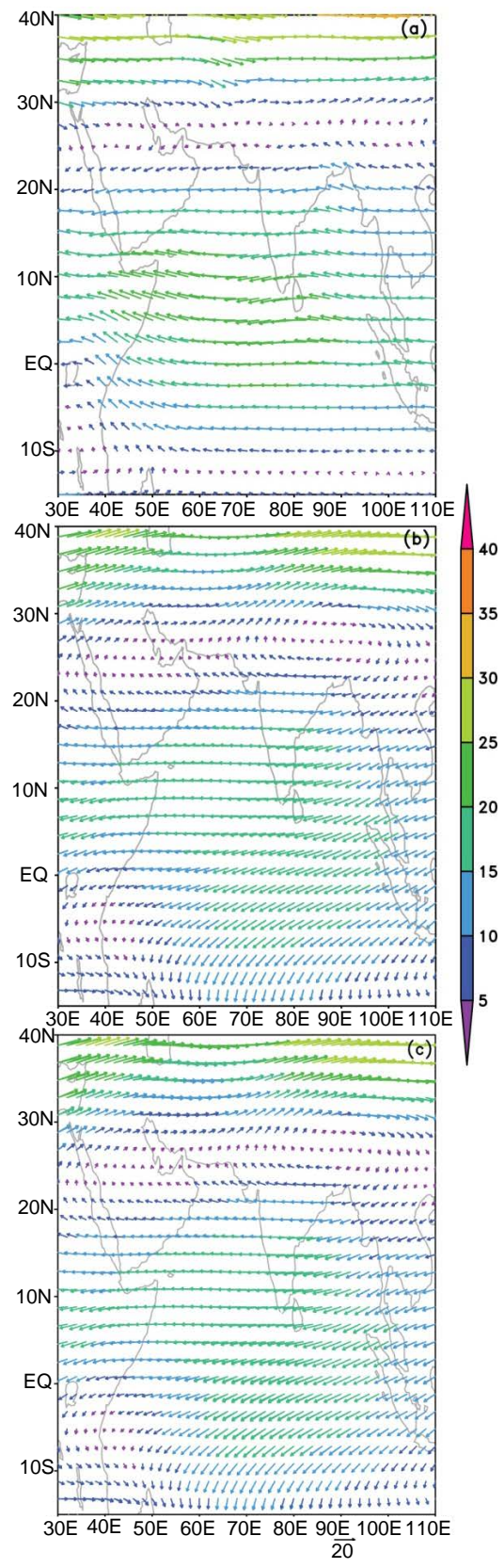
Figure 6. Same as Figure 5 but for vector winds at 200 hPa depicting TEJ.
