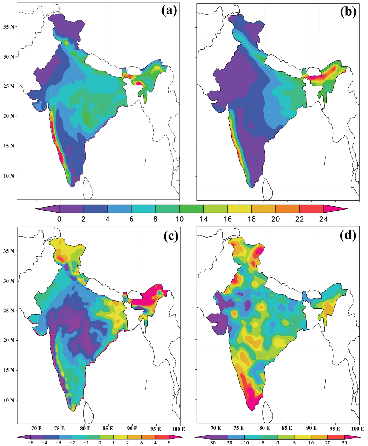
Figure 1. Mean summer monsoon rainfall (June through September, mm/day) over India based on 1951-2000 (a) Observed APHRODITE; (b) Simulated by COSMO-CLM; (c) bias (mm/day); and (d) percentage change for the period 2051-2100 with respect to 1951-2000 under RCP4.5 scenario.
