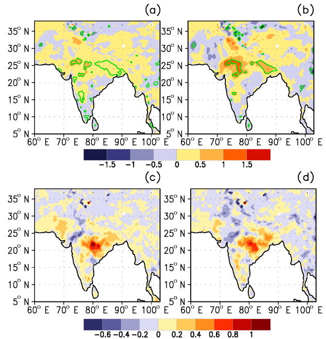
Figure 9. Difference (PLC–HLC) in daily variance of 2 m air temperature in JJAS (in ^\circ\text{C}^2 ; 1982–2008) for (a) daily mean, and (b) daily maximum temperature. Green contour shows significance at the 90 % confidence level. Difference (PLC–HLC) in the 90th percentile of daily 2 m air temperature in JJAS (in ^\circ\text{C} ; 1982–2008), for (c) daily mean, and (d) daily maximum temperature.
