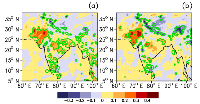
Figure 8. Difference (PLC–HLC) in JJAS-averaged 2 m air temperature (in ^{\circ}\text{C} ; 1982–2008), for (a) daily mean, and (b) daily maximum temperature. Green contour shows significance at the 90% confidence level.
