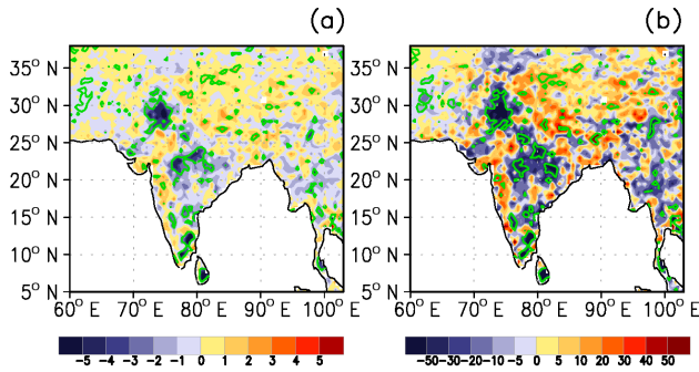
Figure 7. Difference (PLC–HLC) in (a) number of moderate rainfall events during JJAS and (b) total amount of moderate rainfall (in \text{mm day}^{-1} ; 1982–2008). Green contour shows differences significant at the 90% confidence level.
