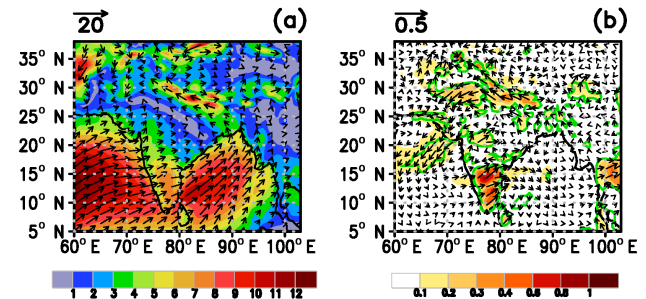
Figure 5. Seasonal (JJAS)-averaged wind at 10 m (in \text{m s}^{-1} ; 1982–2008). (a) Climatological mean (PLC experiment) and (b) difference (PLC–HLC). The shaded color depicts magnitude and arrows show the direction. Green contour shows differences significant at the 90% confidence level.
