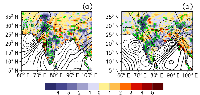
Figure 6. (a) Difference (PLC–HLC experiment) in climatological mean seasonal rainfall (in cm; 1982–2008) shown in shaded color. (b) Same as in (a) but for PLCS–HLCS experiments. Dashed (solid) black contours show the decrease (increase) in velocity potential analog (or the divergent component) of vertically integrated moisture flux qV (from surface–300 hPa). The contour interval is in 1 \times 10^6 \text{ kg s}^{-1} . Green contour shows differences significant at the 90% confidence level.
