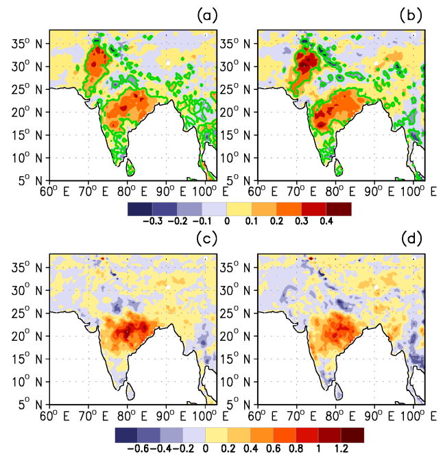
Figure 11. Difference (PLCS–HLCS) in seasonal (JJAS)-averaged 2 m air temperatures (in ^{\circ} C; 1982–2008) for (a) daily mean, and (b) daily maximum temperature. Green contour shows differences significant at the 90 % confidence level. Difference (PLCS–HLCS) in the 90th percentile of daily 2 m air temperature in JJAS (in ^{\circ} C; 1982–2008), for (c) daily mean, and (d) daily maximum temperature.
