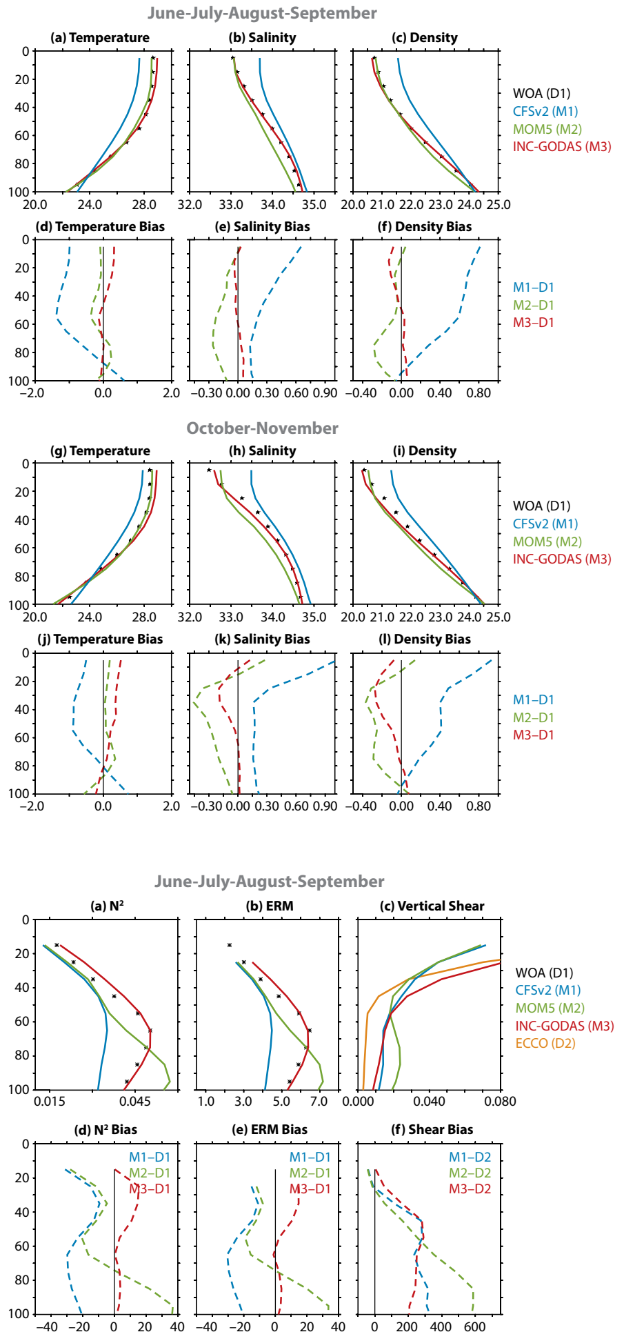
FIGURE 2. Area averaged Bay of Bengal vertical profiles of (a) temperature ( ^{\circ}\text{C} ), (b) salinity (psu), and (c) density ( \text{kg m}^{-3} ) for CFSv2, MOM5, INC-GODAS, and WOA13 during summer (June-July-August-September). (d-f) Plots show respective biases. Similar to June through September, October-November vertical profiles of temperature, salinity, and density and their biases are displayed in (g) to (l). Vertical profiles are displayed for the upper 100 m. Bias is calculated with respect to WOA13.
