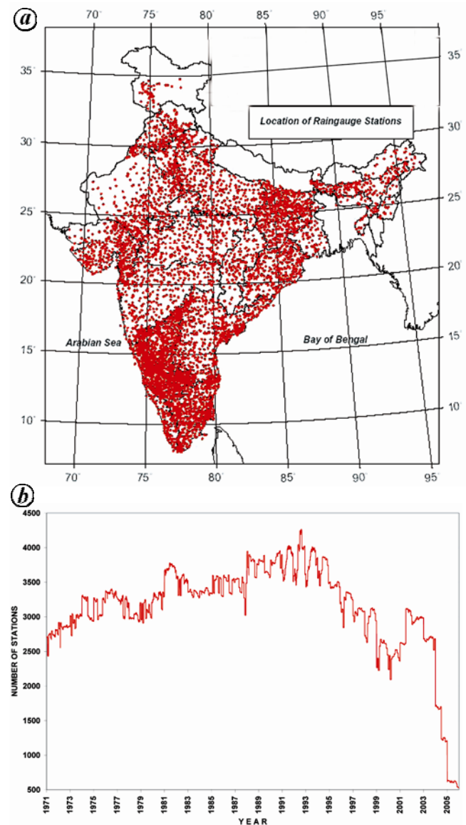
Figure 1. a, Location of rain gauge stations used in the analysis. b, Time series of total number of stations used for rainfall analysis per day for the period 1971–2005.
