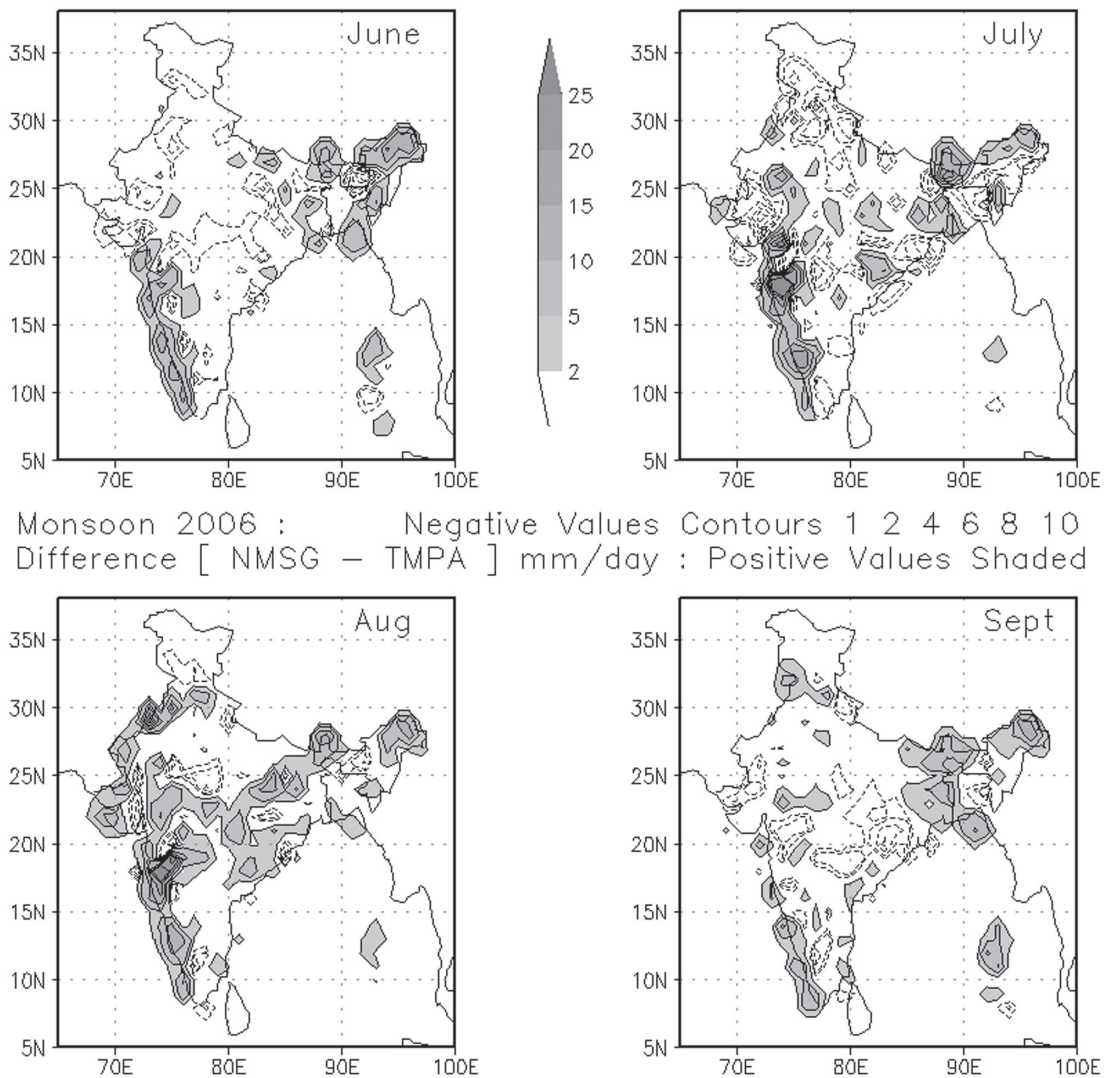
Fig. 4. Difference of analyzed and first-guess (NMSG–TMPA) rainfall (mm day -1 ) for four different months during the 2006 monsoon season.
