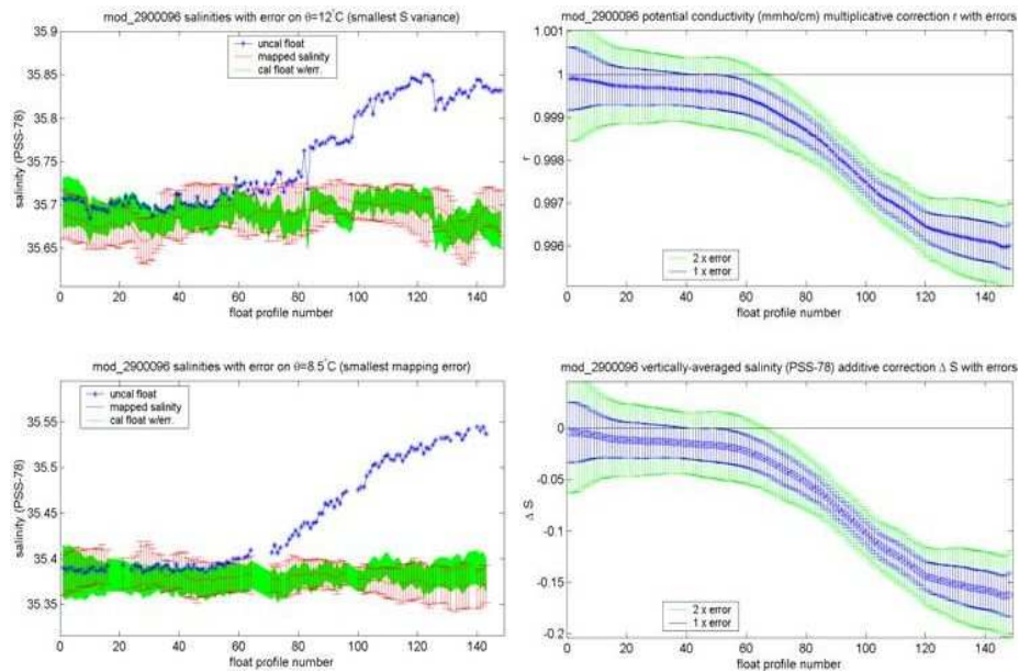
Figure 6: Calibration using WOA alone
