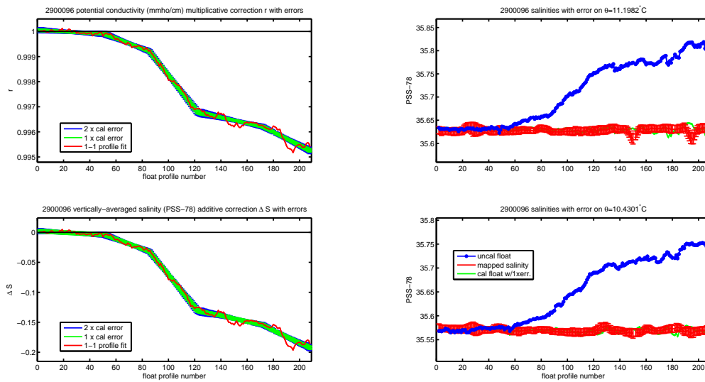
Figure 13: Suggested correction by OW calibration method - Top left panel - suggested correction in terms of conductivity, Bottom left - suggested correction in terms of Salinity. Right panels, depicts quantum of correction applied on 2 isotherms
