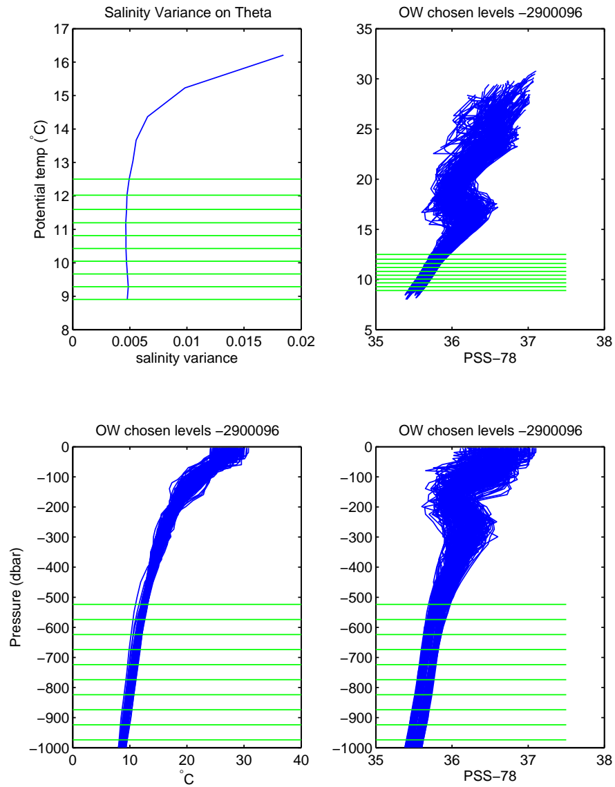
Figure 15: salinity variances on \theta levels & Pressure levels. It also shows the 10 float \theta levels that are chosen for calibration
