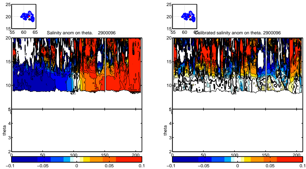
Figure 14: Pre-calibration & Post-calibration salinity anomaly plot on potential temperature
