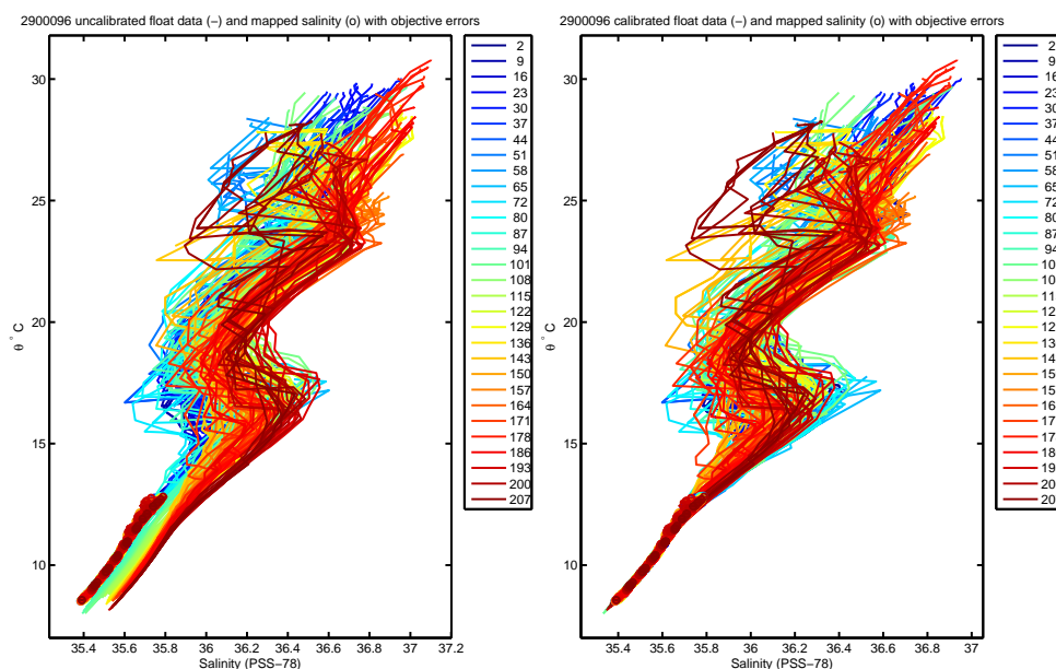
Figure 12: Pre-calibration & Post-calibration TS diagrams of OW method
