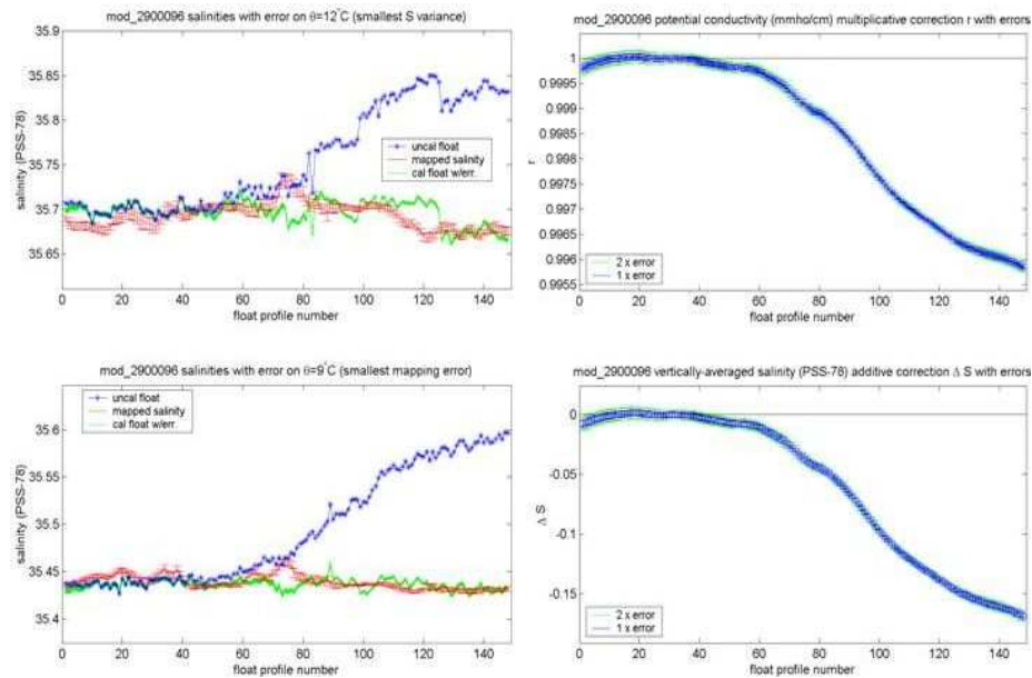
Figure 5: Calibration using only near by Argo profiles
