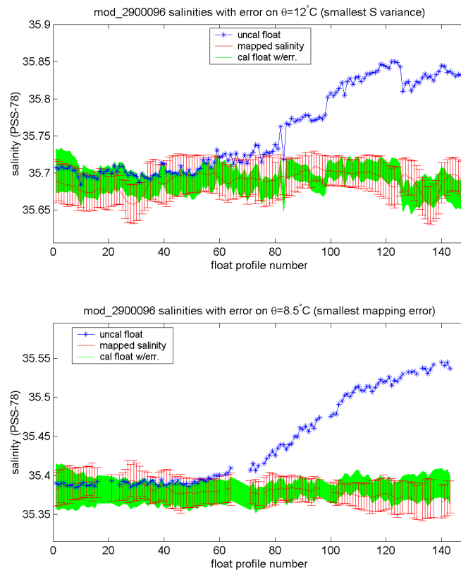
Figure 11: Salinity anomaly plot: Indicates that salinity sensor started drifting from about 65 th profile.
