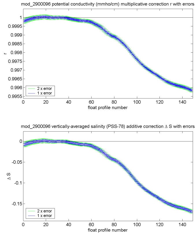
Figure 9: Multiplicative (Top) and Additive (Bottom) corrections applied to the time series)
