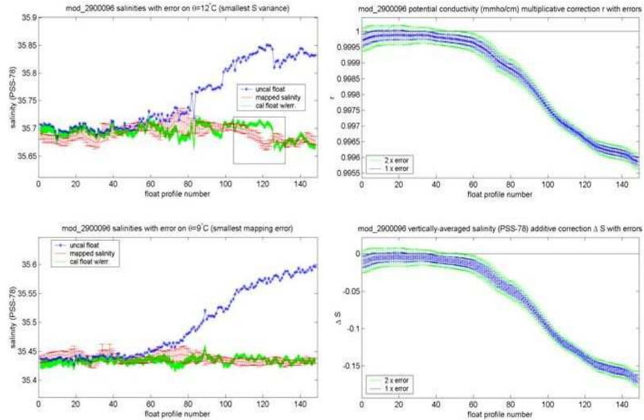
Figure 4: Calibration Using WOA and Argo
