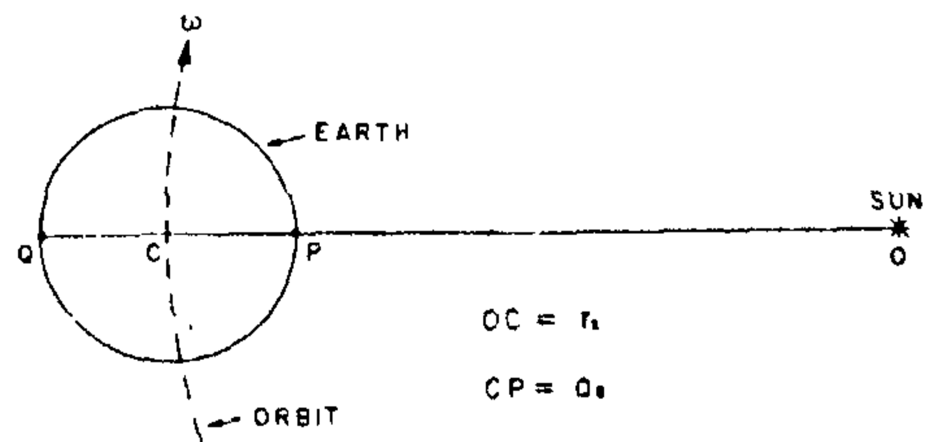
Figure 1. Orbital motion of the earth
