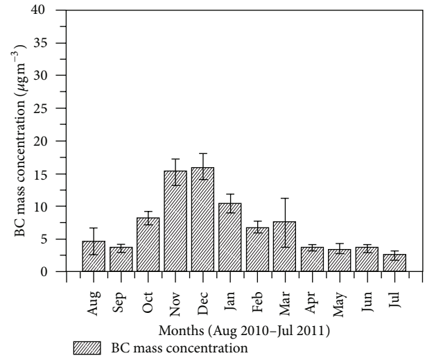
FIGURE 2: Monthly mean variation of BC mass concentration during August 2010–July 2011 over Delhi.
