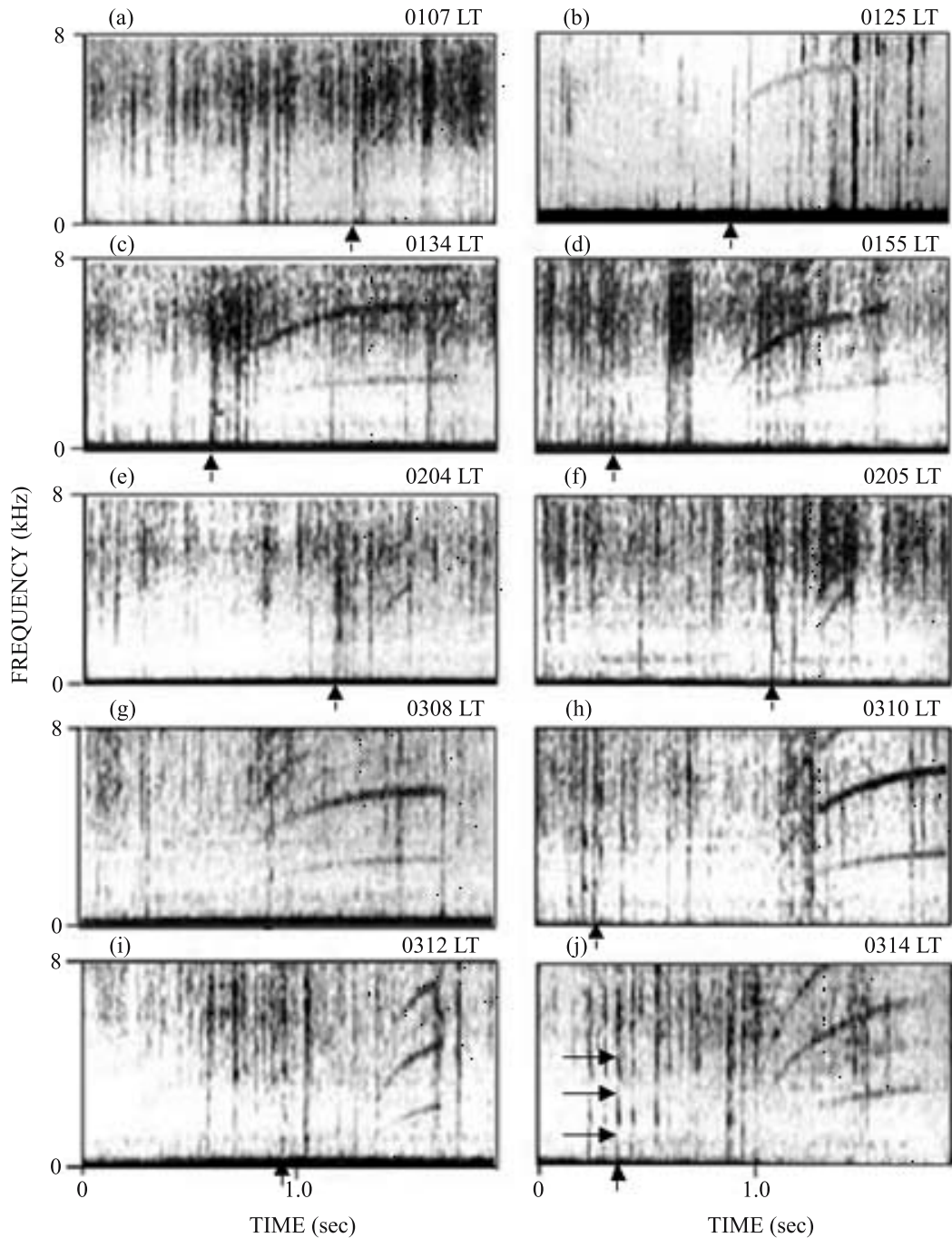
Figure 2. Typical examples of lightning generated sferics along with discrete VLF emissions observed at Gulmarg on 7 March, 1986 (local time). Arrows mark the twecks. The first, second and third harmonics of the twecks are also marked in (j) by arrows on frequency scale.
