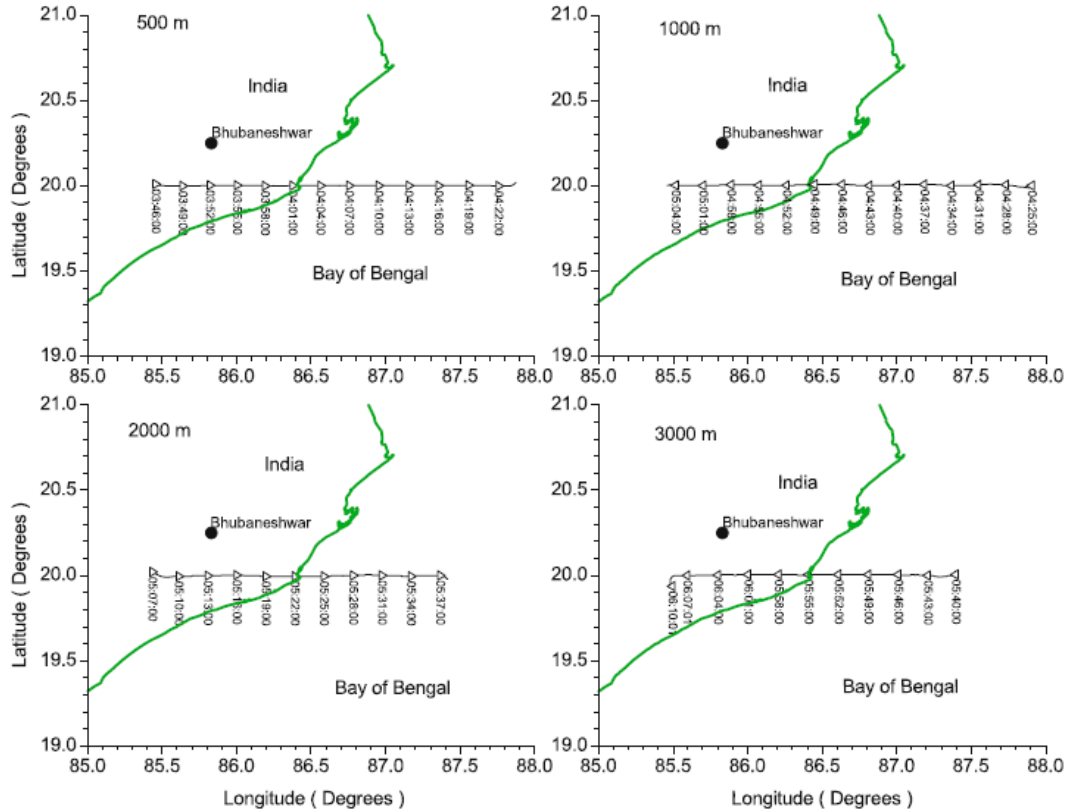
Figure 1. Flight tracks of the aircraft at four different levels. The numbers along the tracks show the mean time of taking an air sample for determination of size distribution.
