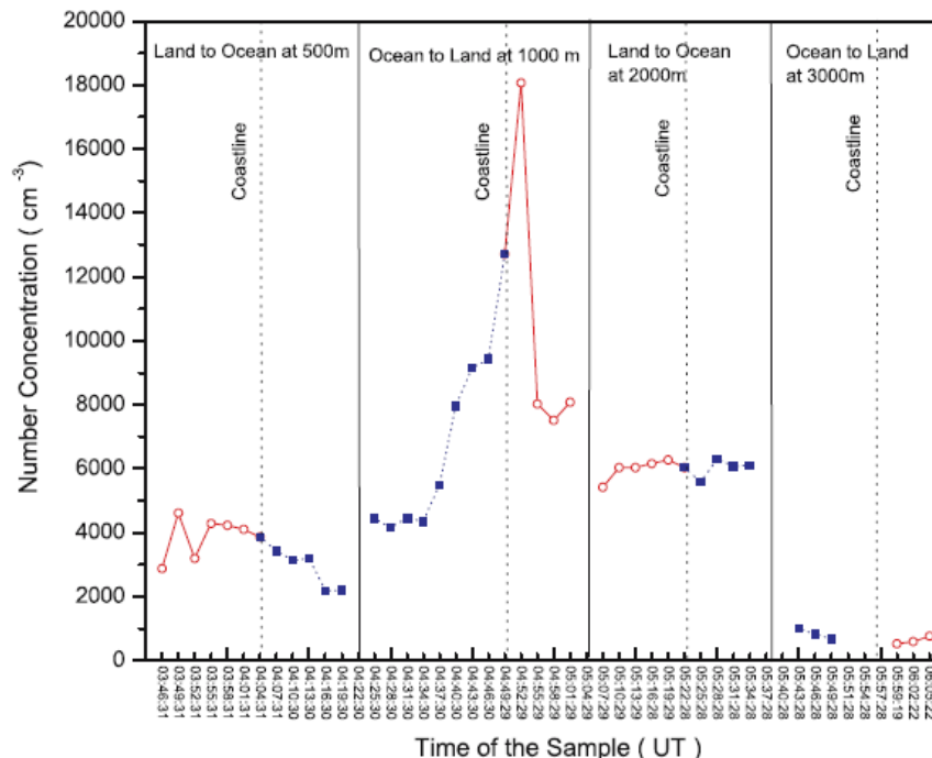
Figure 4. Total number concentration of aerosols along the flight track at different levels. Vertical continuous lines divide the four segments of flight as shown in figure 1.
