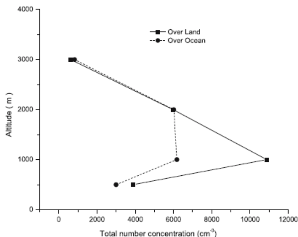
Figure 5. Vertical profiles of total number concentration of aerosols over ocean and over land.
