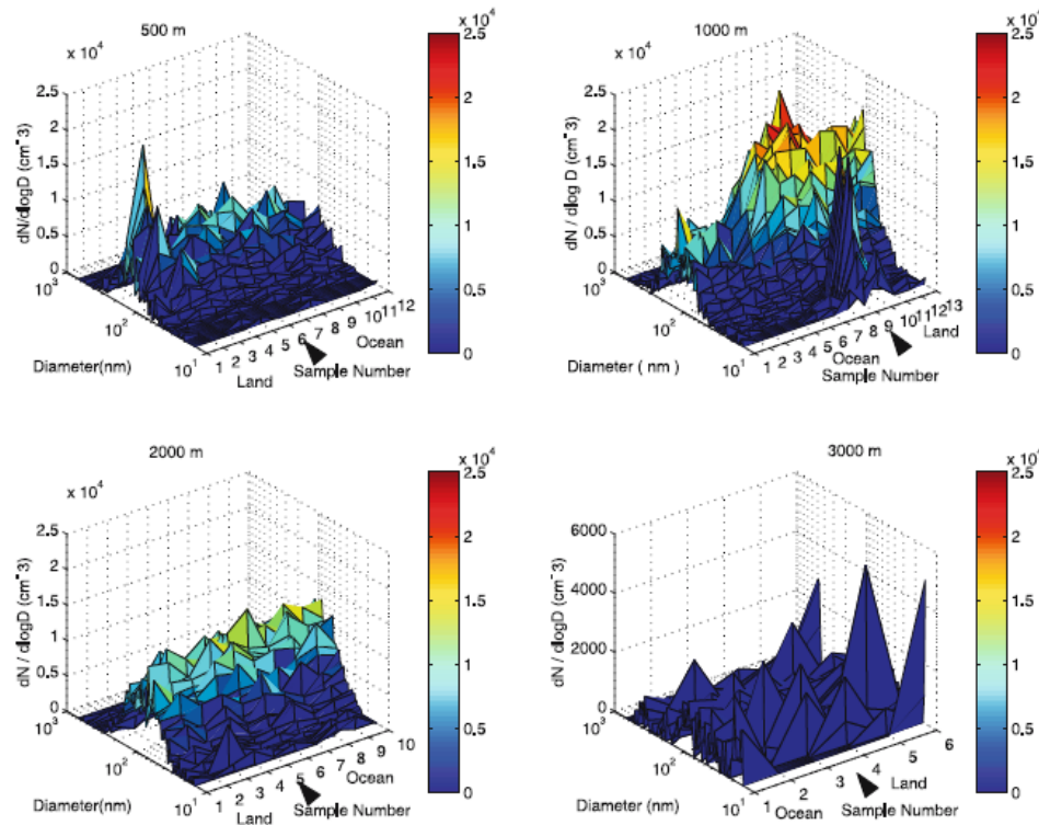
Figure 7. The three-dimensional views of aerosol size distribution obtained at different levels. The arrow on the x axis indicates the position of coastline. Note the change in the vertical scale at 3000 m.
