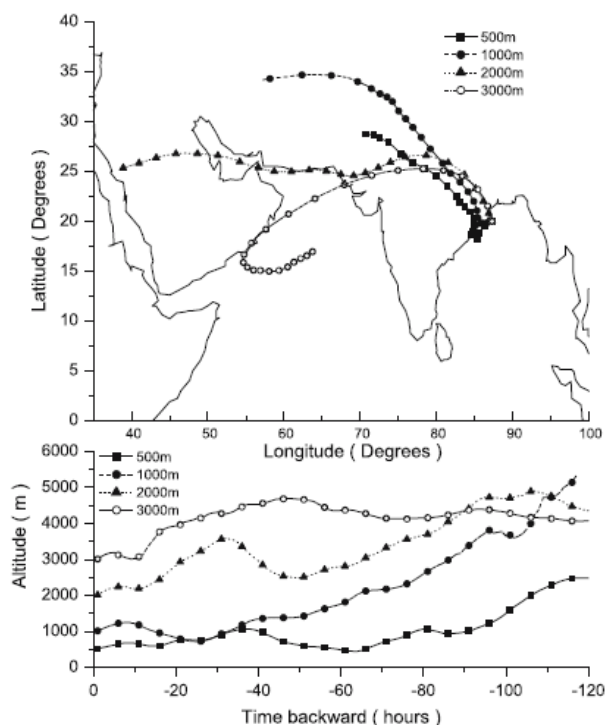
Figure 3. The 5 days back trajectories at different levels at 0400 UT on 25 March, 2006 obtained from NOAA-HYSPLIT model.
