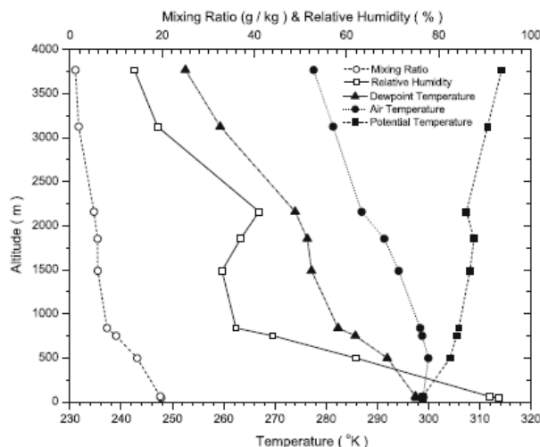
Figure 2. Profiles of air temperature, dewpoint temperature, potential temperature, relative humidity, mixing-ratio calculated from the radiosonde flights made at Bhubaneswar at 00 UT on March 25, 2006.
