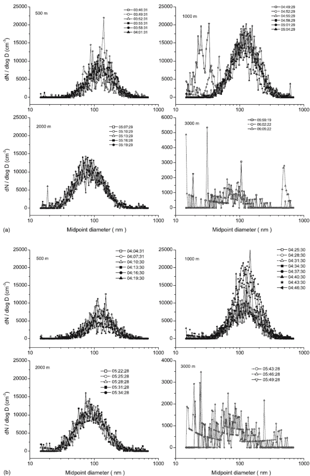
Figure 6. Aerosol number size distributions observed at different times (a) over land and (b) over ocean at different altitudes. Note the change in the vertical scale at 3000 m.
