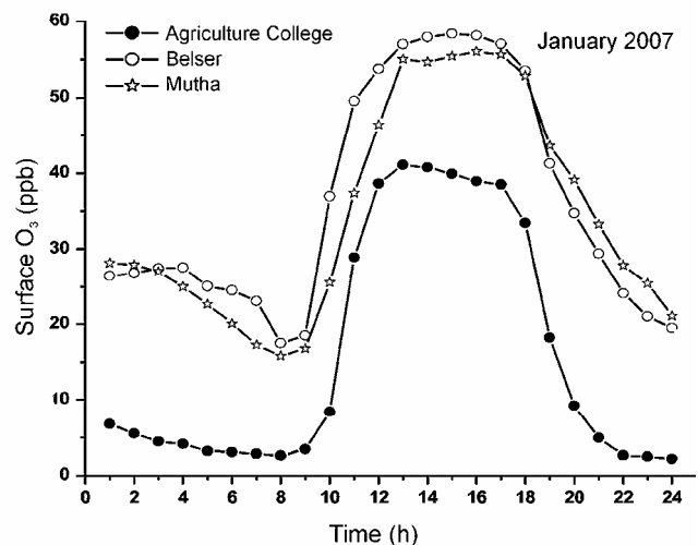
Figure 2. Diurnal variation of surface ozone at the urban and rural locations.
