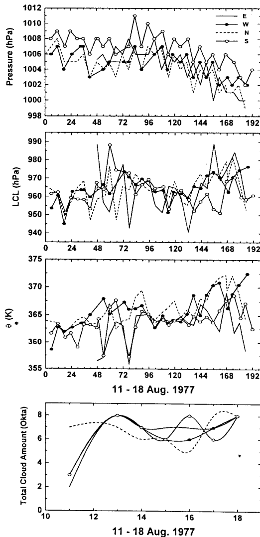
Fig. 6. Daily variation of meteorological parameters at E (solid line), N (dashed line), W (solid line with filled circles) and S (solid line with hollow circles) locations.
