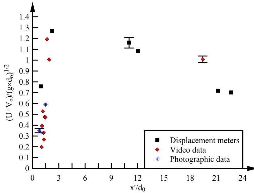
Fig. 4 - Dimensionless celerity of the negative wave as a function of the longitudinal distance for Q = 0.020 \text{ m}^3/\text{s} , h = 0.030 \text{ m} , d_0 = 0.24 \text{ m} - Error bars are included
