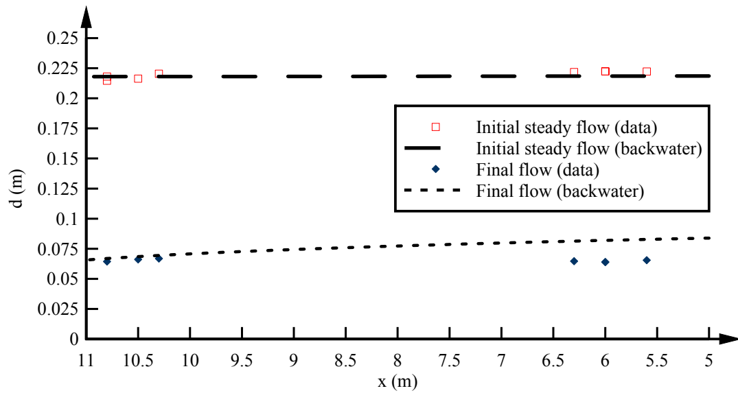
Fig. 2 - Initial steady flow free-surface profile prior to negative surge and final free-surface profile after gate opening - Flow conditions: Q = 0.020 \text{ m}^3/\text{s} , h = 0.030 \text{ m} , steady flow direction from right to left - Comparison between physical data (recorded with acoustic displacement meters) and backwater calculations
