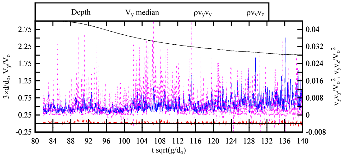
(B) Reynolds stress tensor components \rho v_y^2 and \rho v_y v_z
