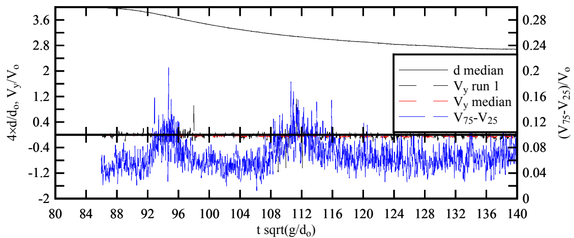
(C) Vertical velocity component V_z at z/d_0 = 0.563
