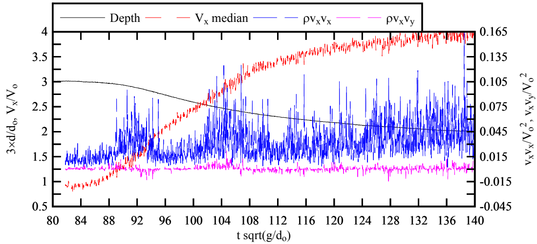
(A) Reynolds stress tensor components \rho v_x^2 and \rho v_x v_y
