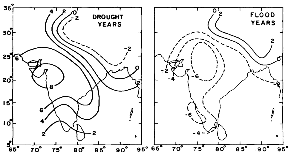
FIG. 7. Surface pressure departure ( 10^{-1} mb) during the southwest monsoon season.
