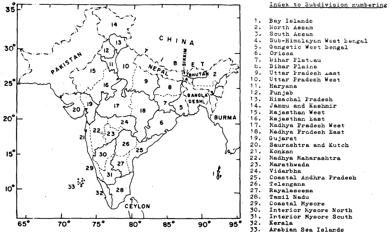
FIG. 1. Meteorological subdivisions of India as of 1 January 1971.
