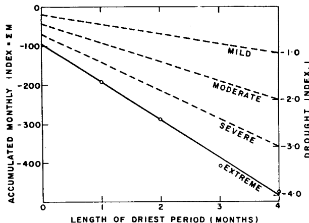
FIG. 2. Accumulated moisture index during the periods of various lengths.
