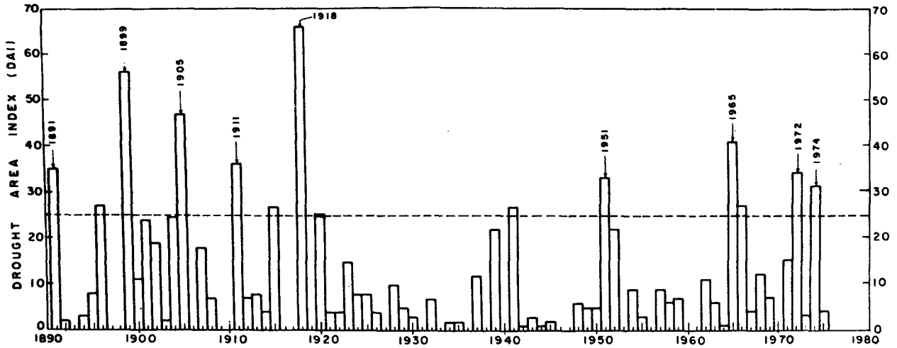
FIG. 4. Drought Area Index (DAI) from 1891-1975.
