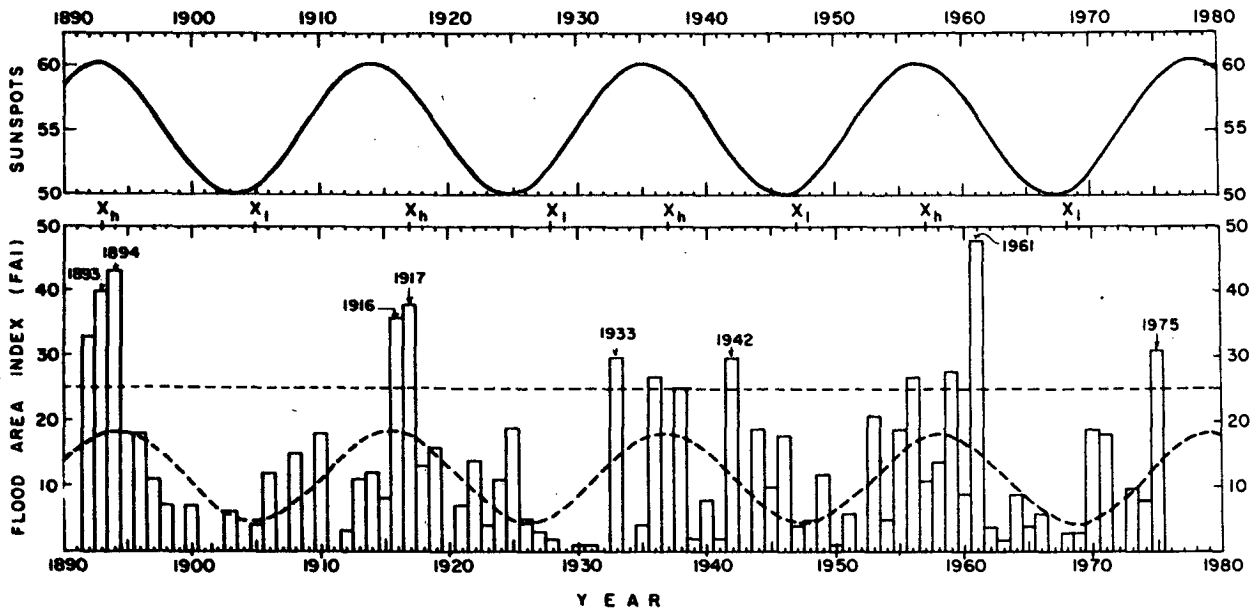
FIG. 5. Lower: Flood Area Index (FAI) from 1891-1975, the years of high-amplitude sunspots maximum ( X_h ), the years of low-amplitude sunspots maximum ( X_l ), and a wave of 21-year period in the FAI series. Upper: A wave of 21-year period in sunspots from 1891-1975.
