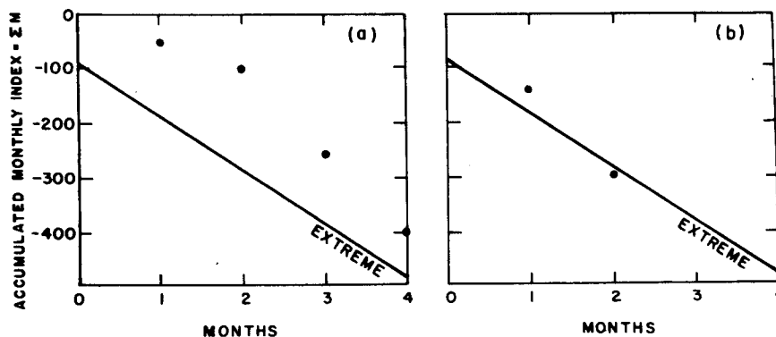
FIG. 3. An illustration of misleading cumulative procedure. (a) Two relatively dry months followed by two very dry months; (b) two very dry months alone.
