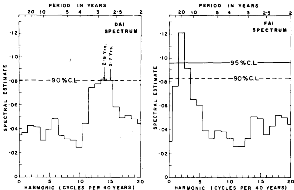
FIG. 6. Power spectra of DAI and FAI series.
