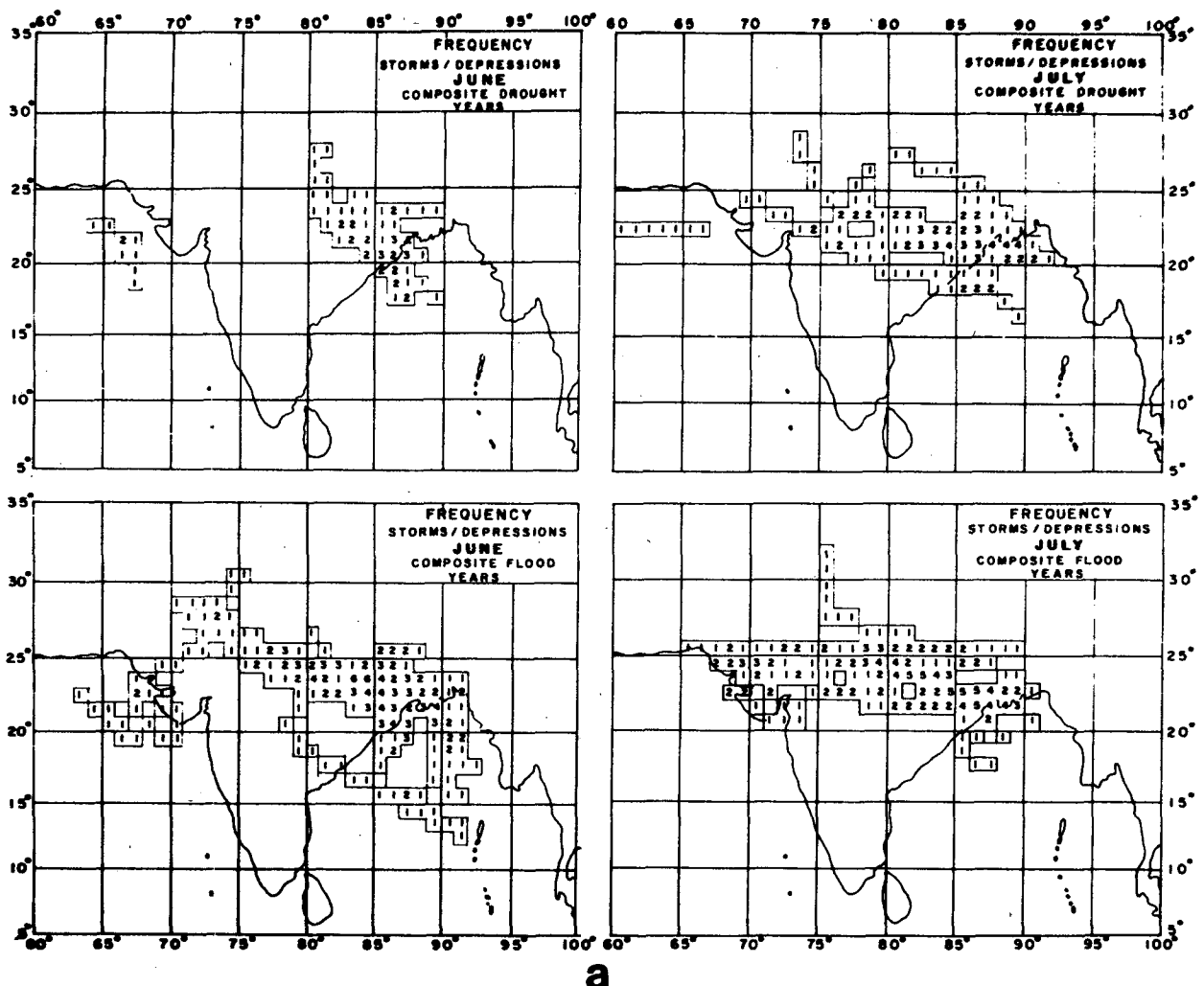
FIG. 8a. Frequency of storms and depressions (June and July).
