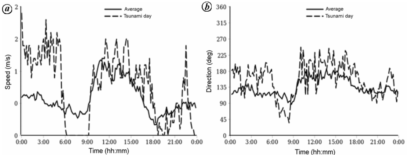
Figure 6. Diurnal variation of (a) wind speed (m/s) and (b) wind direction during the tsunami day (26 December 2004). The solid line is the average diurnal variation of the same parameter during the clear-sky days.
