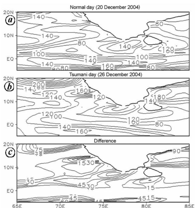
Figure 4. Spatial structure of latent heat flux during (a) normal day (20 December 2004), (b) tsunami day and (c) tsunami–normal day, i.e. the difference.
