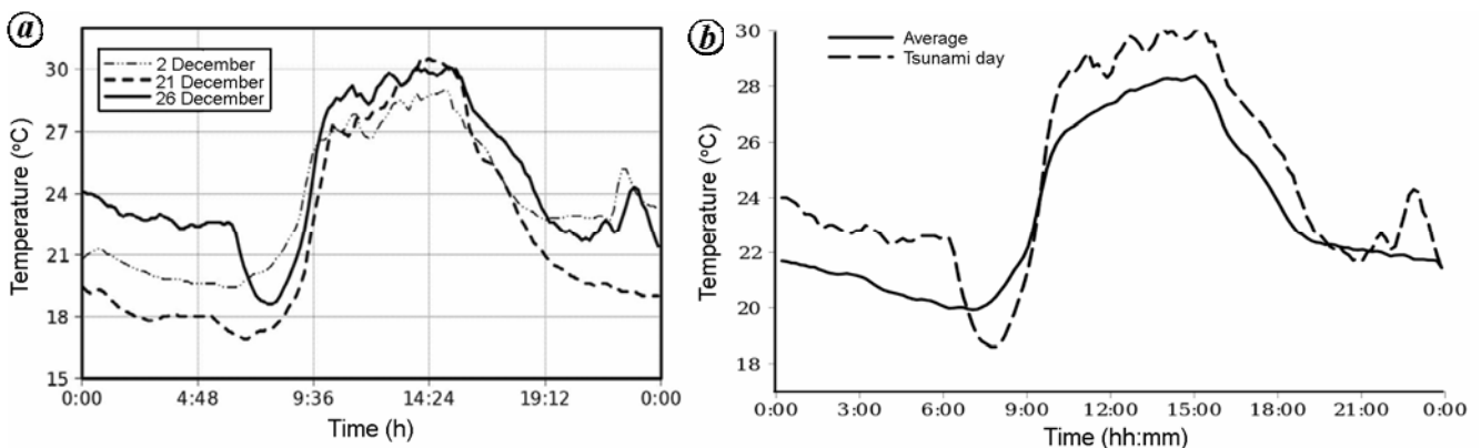
Figure 3. a , Comparison of diurnal variation of air temperature (AT) during the tsunami day (26 December 2004) and two other normal days to indicate the abnormal variation. b , Diurnal variation of AT during the tsunami day. The solid line is the average diurnal variation of the same parameter during the clear-sky days.
