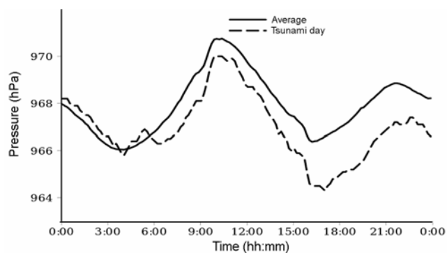
Figure 5. Diurnal variation of surface pressure during the tsunami day (26 December 2004). The solid line is the average diurnal variation of the same parameter during the clear-sky days.
