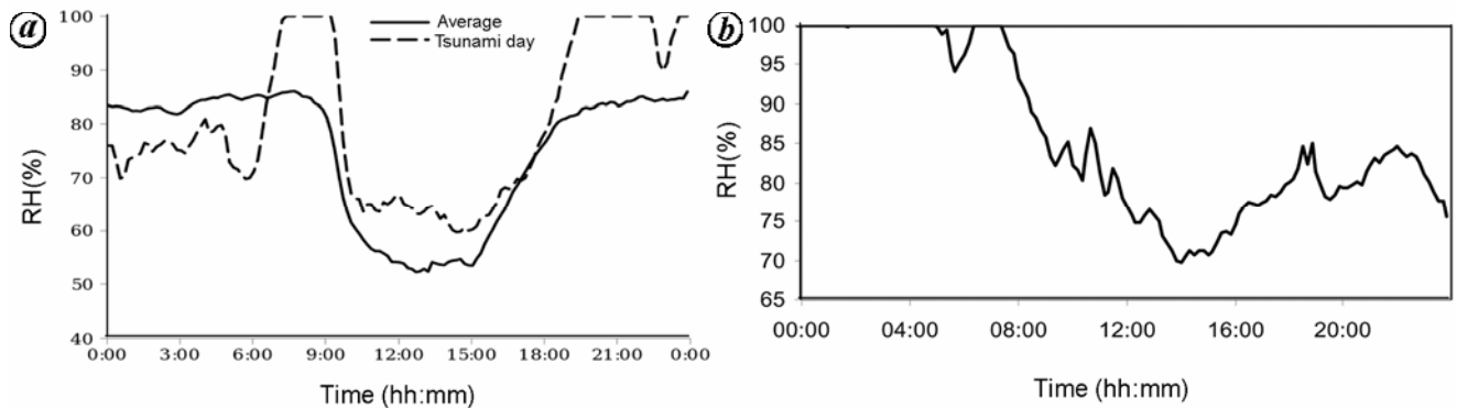
Figure 2. a , Diurnal variation of relative humidity (RH) during the tsunami day, i.e. 26 December 2004 (shown as dashed line). The solid line is the average diurnal variation of the same parameter during the clear-sky days. b , Variation of RH recorded at Braemore station on the previous day, i.e. 25 December 2004.
