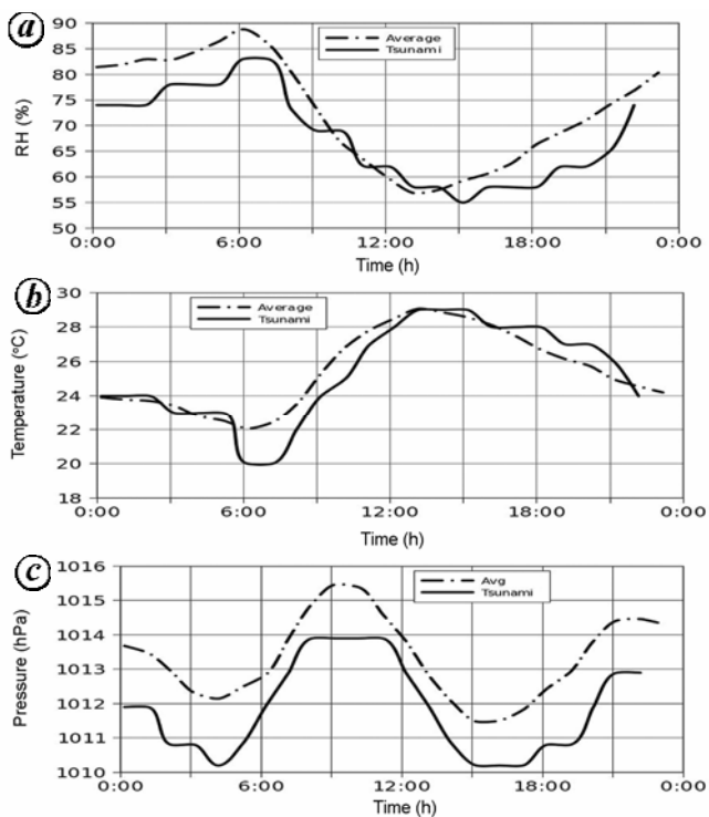
Figure 7. Diurnal variation of (a) relative humidity (%), (b) air temperature (°C) and (c) surface pressure (hPa) during the tsunami day (26 December 2004). The dotted line is the average diurnal variation of the same parameters during the month of December.
