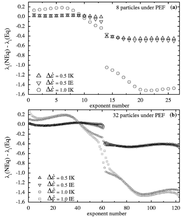
FIG. 6. Differences between the values of the exponents in a nonequilibrium steady-state for PEF [\lambda_i(\text{NEq})] and the corresponding value at equilibrium [\lambda_i(\text{Eq})] . In (a), systems of 8 particles under isokinetic and isoenergetic dynamics are shown. In (b), systems of 32 particles are depicted: \Delta\dot{\epsilon} indicates the shift between equilibrium and nonequilibrium elongational rates and IK/IE shows the constrained dynamics.
