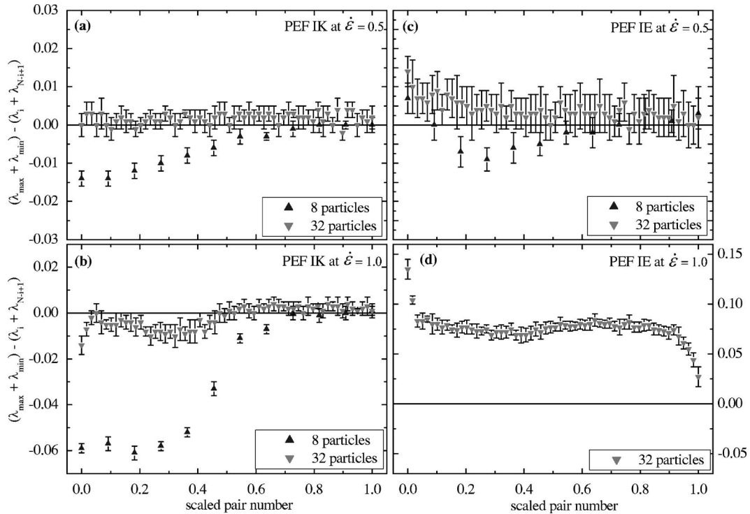
FIG. 7. Differences between the sum of maximum and minimum Lyapunov exponents and the sums of scaled pairs for systems of eight and 32 particles under PEF at \dot{\epsilon}=0.5 and 1.0. The values of the differences are indicated by filled triangles with error bars. Systems under isokinetic dynamics are in (a) and (b) and under isoenergetic dynamics in (c) and (d). Plots at \dot{\epsilon}=0.5 have the same scale; plots at \dot{\epsilon}=1.0 have different scales. The error bars represent twice the standard error of the mean of ten independent runs.
