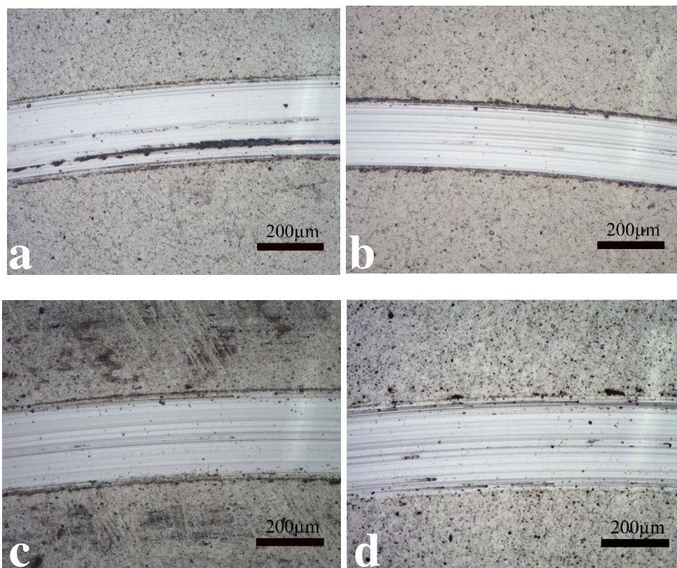
Fig. 10. Optical image of the wear track of the coating deposited at (a) - 40 V, (b) - 65 V, (c) - 100 V and (d) -150 V.
