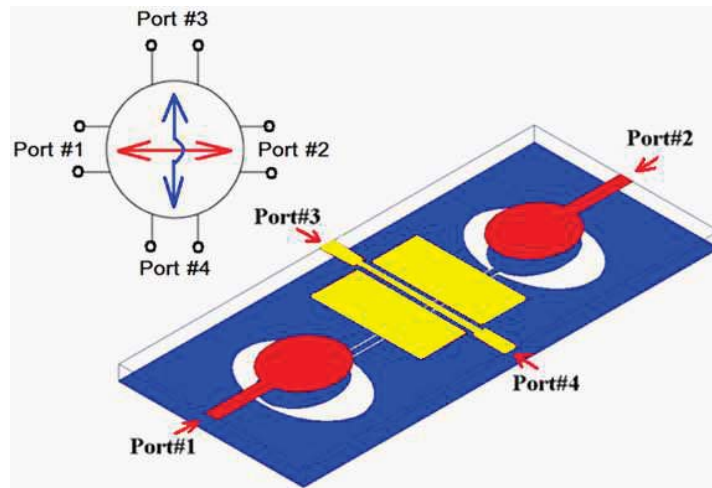
Figure 5. Structure of the new crossover incorporating the double interconnect and finite width CPW crossing line.
