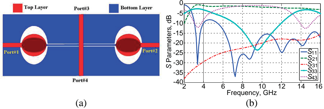
Figure 4. (a) Simulated structure of the crossover incorporating the double interconnect and the microstrip line. (b) Simulation results for its scattering matrix parameters.
