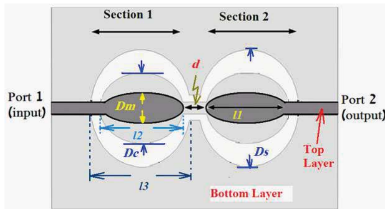
Figure 1. Configuration of double vertical interconnect [18].
