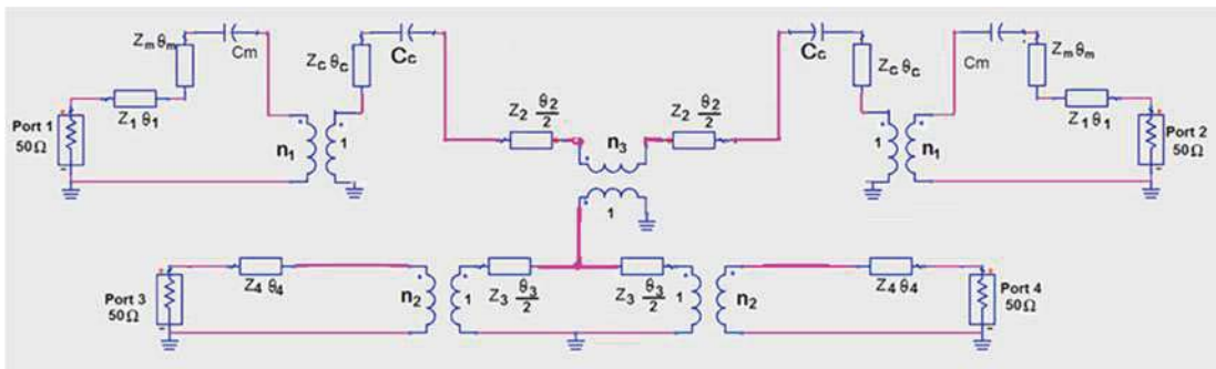
Figure 6. Equivalent circuit model of the proposed crossover.
