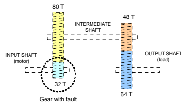
Fig. 7 two stage gearbox with a missing tooth on the input shaft
