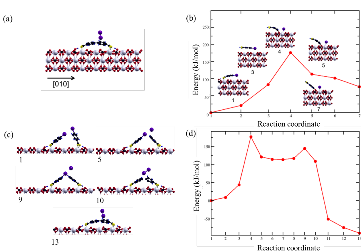
Figure 7. (a) IBA dimer configuration, final product after a dehalogenation reaction. (b) and (c,d) Minimum paths and energy barriers of two main mechanisms of IBA dehalogenation on calcite (10.4) [44]: (a) Independent mechanism: single molecules dehalogenate and chemisorb on the substrate before dimerization. The iodine adsorption is also visible. (c,d) Cooperative mechanism of double dehalogenation, as described in the text. In this case, the key factors facilitating the reaction are the two asynchronous dehalogenations, the exchange and sharing of the iodine atoms during the detachments from the molecules, and the I_2 recombination. Reaction coordinate numbers correspond
