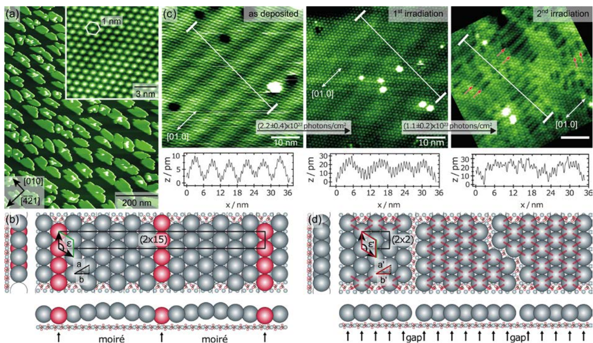
Figure 9. (a) Image showing C_{60} islands on calcite (10.4). Image adapted with permission from [41]. (b) Proposed model explaining the superstructure and the origin for the observed moiré pattern. (c) Image series showing the changes induced upon irradiation of the film with a 405 nm laser diode. (d) Model explaining the preferential reaction direction by a reduction in the lattice mismatch. Images (b) to (d) adapted with permission from [46].
