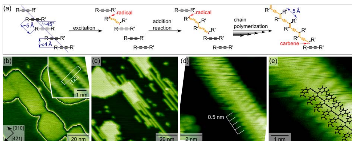
Figure 10. (a) Diacetylene reaction scheme. (b) Image showing the as-deposited structure of 3BBA on calcite (10.4). (c) Image showing the structural changes upon annealing the sample to 485 K. (d) Zoom in a molecular row. (e) Row structure with superimposed DFT model. Images (b) to (e) adapted with permission from [47].
