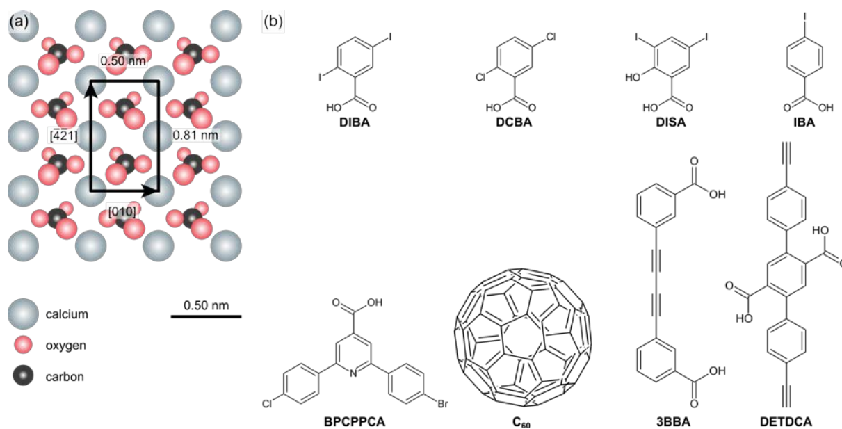
Figure 1. (a) Model of the calcite (10.4) cleavage plane. The surface unit cell consists of two calcium ions and two carbonate groups. (b) Compilation of the molecules discussed in this review. The scale bar applies to both subsets.
