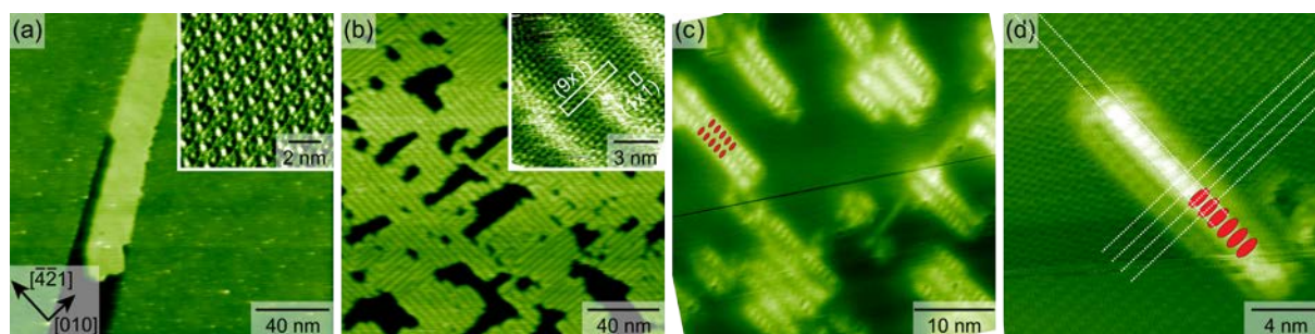
Figure 4. (a) Calcite surface after deposition of IBA. Images reprinted (adapted) with permission from [72]. Copyright (2013) American Chemical Society. (b) Upon annealing to about 500 K, the intermolecular hydrogen bonded network breaks and a wetting layer is formed that is governed by hydrogen bonds between the molecules and the substrate. (c) Structure as obtained after annealing to 580 K. (d) High-resolution image showing a molecular row and the atomic structure of the surface simultaneously. BPDCA molecules are superimposed as ellipses to illustrate the envisioned side-by-side alignment of the dimerized IBA molecules. Images (b) to (d) reprinted (adapted) with permission from [43]. Copyright (2011) American Chemical Society.
