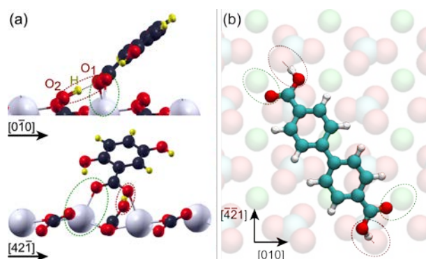
Figure 2. Binding configuration of a carboxylic acid group onto calcite (10.4) in an upright position (a) and lying flat (b). Note that (a) is based on DFT calculations as published in [51], while (b) is a sketch based on the calculations shown in [50]. Reprinted (adapted) with permission from [50]. Copyright (2016) American Chemical Society.
