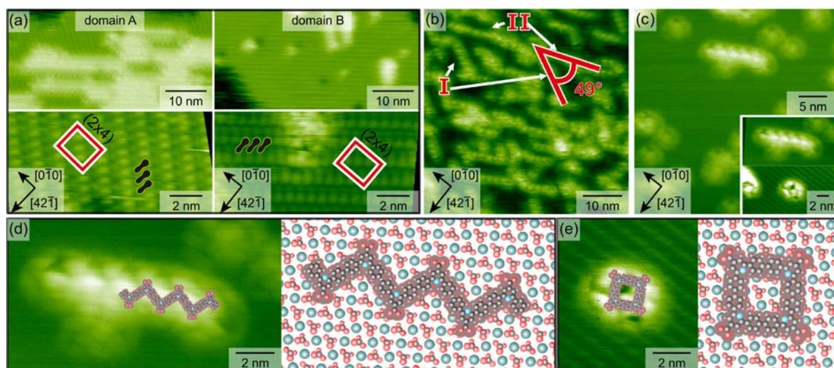
Figure 8. (a) As-deposited structure of BPCPPA on a calcite (10.4) surface held at room temperature. Two mirror domains of (2 \times 4) islands are formed. (b) After annealing to 570 K, a first structural
