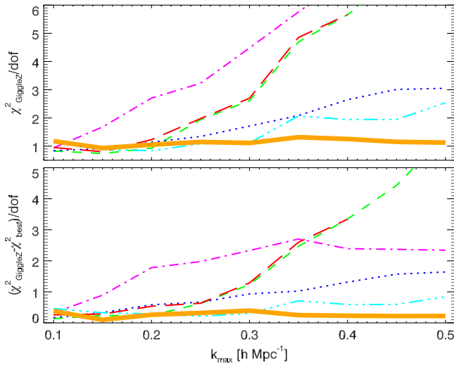
FIG. 3 (color online). Upper : Reduced \chi^2 of models A)–F) fitted to the N -body simulation halo catalogue for the Gigglez fiducial cosmology values. In absence of systematic errors the models should recover the input cosmology with \chi^2/\text{dof} = 1 . Lower : Difference in reduced \chi^2 values when using the Gigglez fiducial cosmological parameters and the best fit values. The models are (A) blue dotted, (B) green dashed, (C) magenta dot-dashed, (D) cyan triple dot-dashed, (E) red long dashed, (F) thick orange solid.
