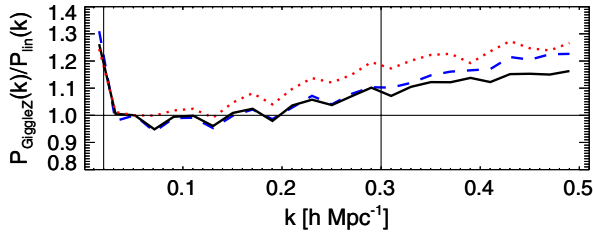
FIG. 1 (color online). The ratio between the simulated WiggleZ halo power spectrum (from GiggleZ) and the corresponding linear power spectrum (normalized to the first bin) at z = 0.2 (blue dashed) and z = 0.6 (black solid) and for luminous red galaxies (dotted red). The vertical lines indicate our fitting range of k = 0.02\text{--}0.3h \text{ Mpc}^{-1} . Nonlinear corrections are clearly less significant for the high-redshift, low-bias WiggleZ halos than at lower redshifts.
