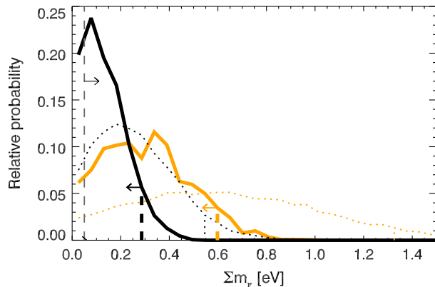
FIG. 5 (color online). The relative probability distribution of \sum m_\nu , from fitting model F) with k_{\max} = 0.3h \text{ Mpc}^{-1} for WMAP (dotted orange), WiggleZ + WMAP (solid orange), WMAP + BAO + H_0 (dotted black) and WiggleZ + WMAP + BAO + H_0 (solid black). The dashed grey line is the lower limit from oscillation experiments, and the vertical lines are 95% confidence upper limits.
