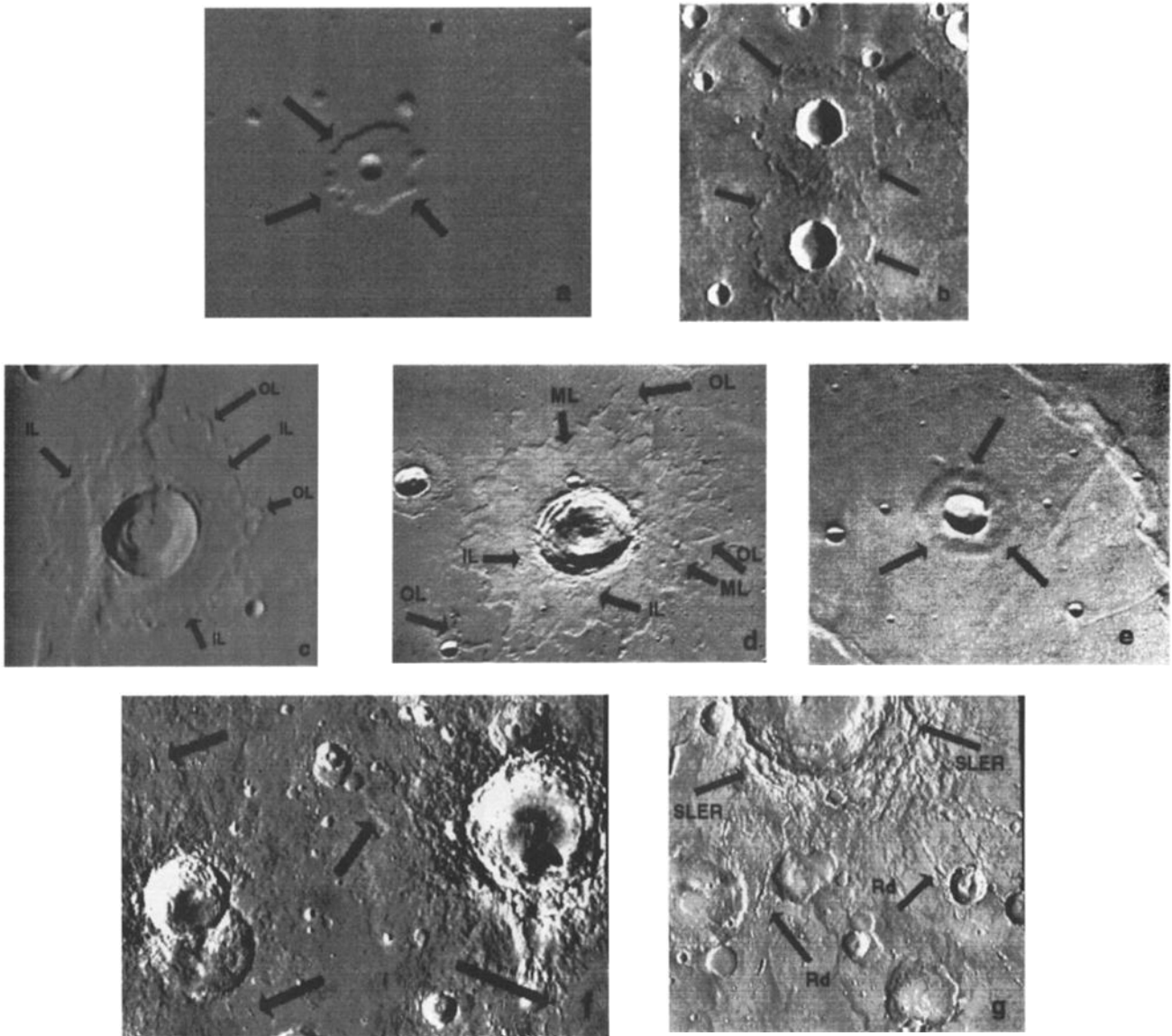
Figure 1. Examples of the new ejecta morphology classifications recommended by the Mars Crater Morphology Consortium. Arrows point to the distinguishing ejecta features. (a) A 1.5-km-diameter pedestal (Pd) crater, located at 11.4°N, 161.5°W, (Viking Orbiter image 886A09). (b) Two single-layer ejecta rampart sinuous (SLERS) craters. The top crater is 18.1 km in diameter and located at 8.80°N, 72.13°W. The bottom crater is 18.9 km in diameter and located at 7.96°N, 72.16°W (Viking Orbiter image 858A56). (c) A 9.6-km-diameter double-layer ejecta rampart sinuous (DLERS) crater, located at 21.42°N, 79.02°W (Viking Orbiter image 555A24). IL identifies the inner ejecta layer; OL denotes the outer ejecta layer. (d) A 33.9-km-diameter multiple-layer ejecta rampart sinuous (MLERS) crater, located at 26.59°N, 38.55°W (Viking Orbiter image 827A01). IL indicates the inner ejecta layer, ML identifies the middle ejecta layer, and OL denotes the outer ejecta layer. (e) A 7.7-km-diameter single-layer ejecta pancake circular (SLEPC) crater, located at 26.10°S, 69.04°W (Viking Orbiter image 608A29). (f) Single-layer ejecta radial (SLERd) craters. The large crater on the left is 75.3 km in diameter and located at 24.36°N, 10.79°W (MDIM image Mg25n012). (g) A 107.2-km-diameter single-layer ejecta rampart circular radial (SLERCRd) crater, located at 32.32°N, 337.9°W (MDIM image Mg30n337). Rd indicates the radial component of the ejecta blanket, while SLER identifies the single-layer ejecta rampart portion of the blanket.
