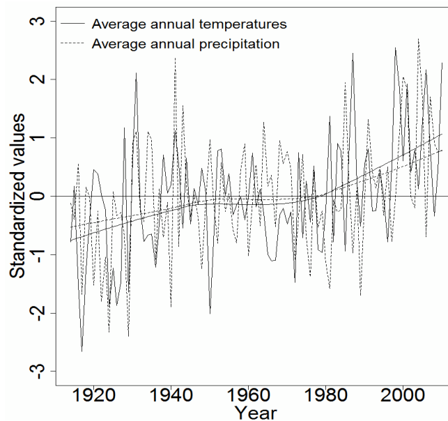
Figure 1. Mean annual temperature and precipitation (each value was standardized by subtracting the population mean and then dividing by the standard deviation) from 1915 to 2008 in the sampling area. General trends are illustrated using loess smoothing lines.
