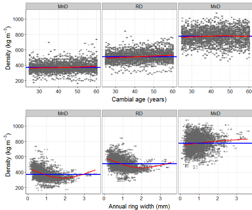
Figure A1. Minimum, mean and maximum ring density against cambial age and ring width. The red lines represent the mean predictions from model 1 for each density component (Tables 3–5), and the blue lines represent the overall mean values.
