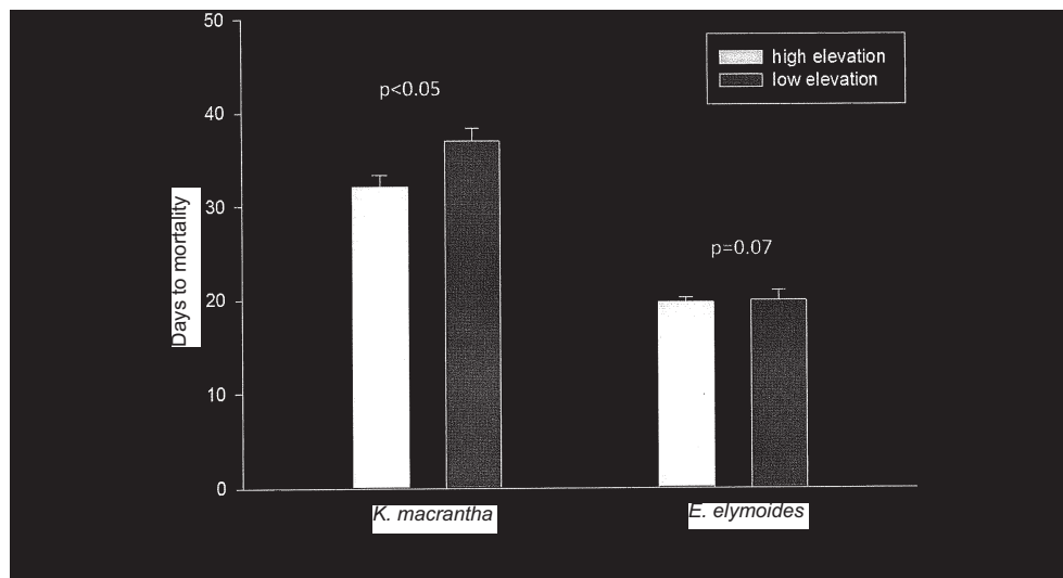
Fig. 2. Average number of days to aboveground mortality in plants from high- and low-elevation populations of Koeleria macrantha and Elymus elymoides under simulated drought conditions. Error bars represent standard error.
