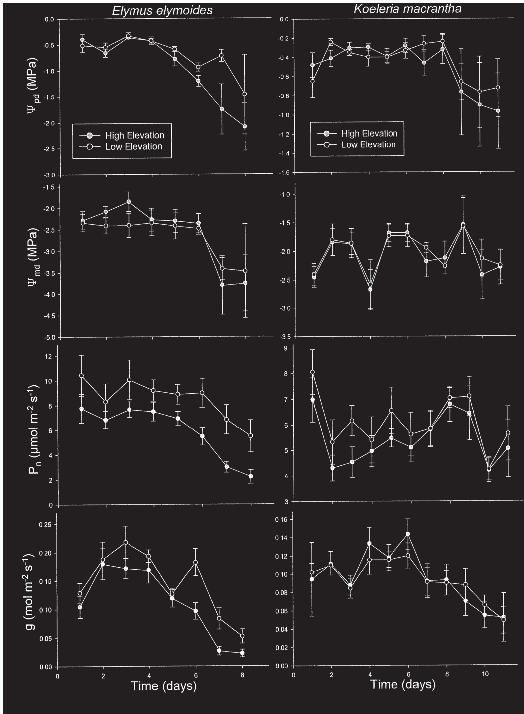
Fig. 1. Response of gas exchange traits to simulated drought, as represented by days since watering. Plants are from high-elevation (solid points) and low-elevation (open points) populations of 2 grass species— Koeleria macrantha and Elymus elymoides —in northern Arizona. Traits are predawn leaf water potential ( \Psi_{pd} ), midday leaf water potential ( \Psi_{md} ), net photosynthetic rate ( P_n ) and stomatal conductance ( g ). Means are depicted with bars representing one standard error around the mean.
