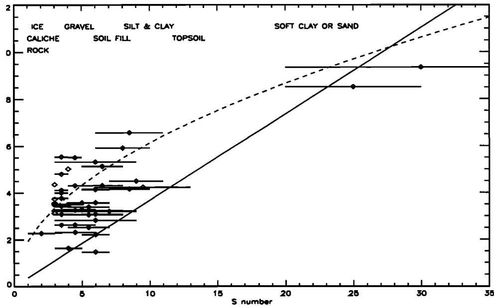
Figure 6. Expected penetration depth, assuming impact velocity of 200 m/s and forebody mass of 850 g as a function of soil hardness S . Solid line is formula by Young [1967; 1997]; dashed line is that in the text. Diamonds with error bars indicate results from New Mexico tests. Upper part of graph indicates typical soil types associated with various S number ranges.
