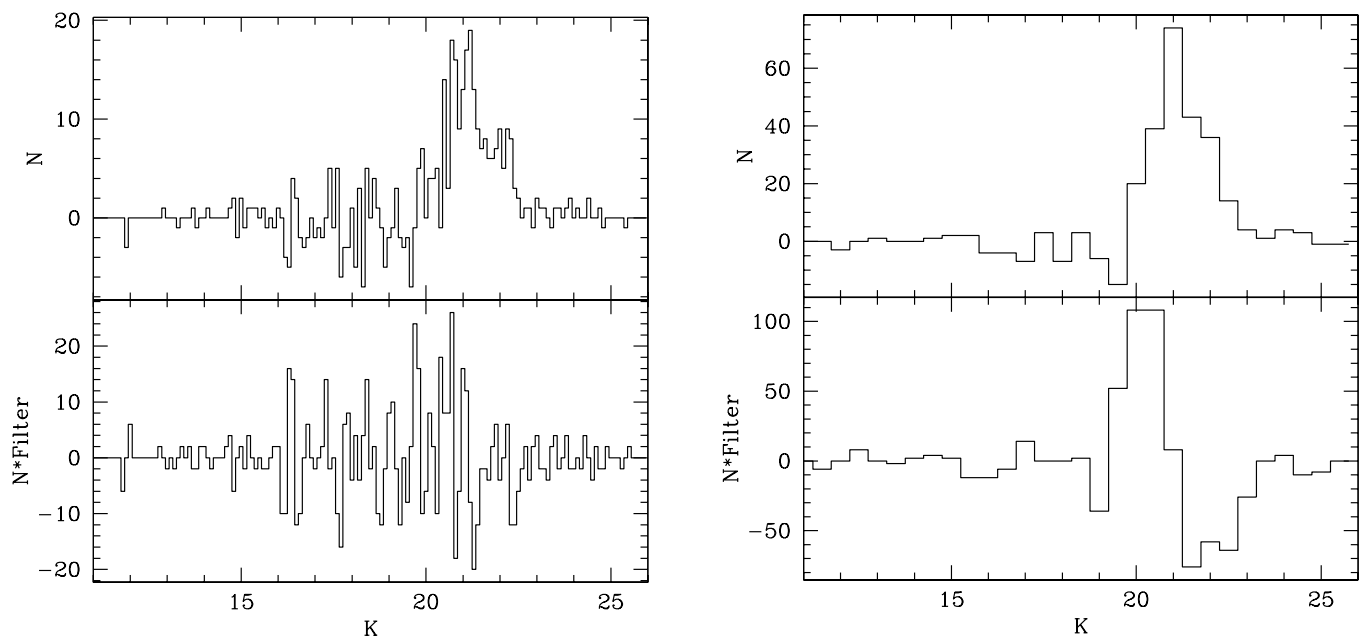
FIG. 5.—Background-corrected K -band luminosity function for HIZSS 3 field before ( top panels ) and after ( lower panels ) convolution with Sobel [-2, 0, +2] edge detection filter. Two bin sizes are shown: 0.1 mag ( left ) and 0.5 mag ( right ).
