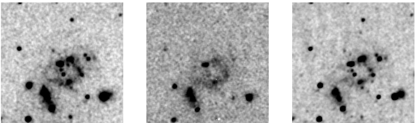
FIG. 3.—Cut-out images of the H II region detected by MHK03. From left to right: J_s , \text{Pa}\beta , and K_s . North is up, and east is to the left. Each image is 22'' \times 22'' .
