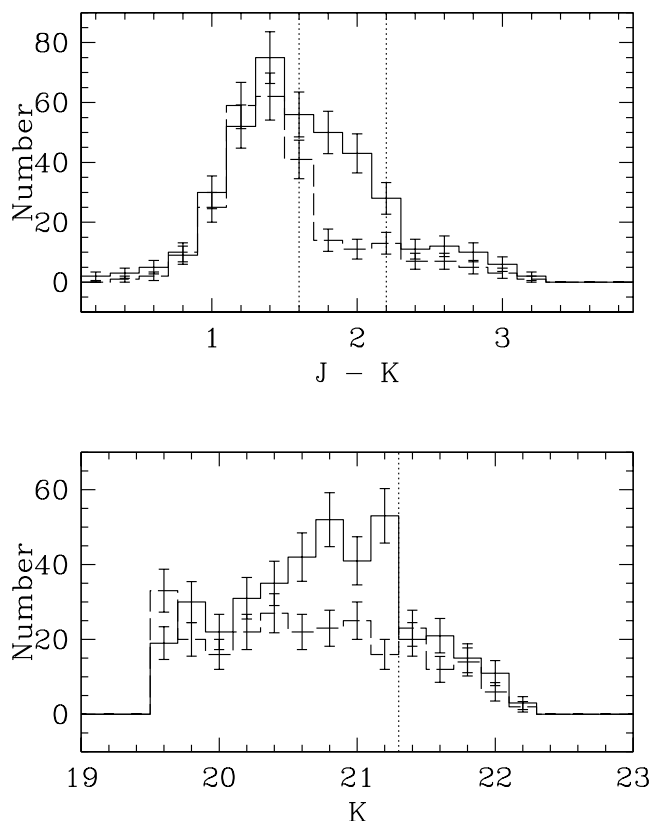
FIG. 7.—Color and luminosity distributions used to select RGB candidates. Only stars with K > 19.5 and \sigma_{J-K} \leq 0.2 are shown. Neither color nor luminosity are corrected for foreground extinction. In both panels, the solid histogram shows the HIZSS 3 stellar distribution, while the dashed line shows the distribution of objects in the reference field. In the color distribution panel, the vertical dashed lines delineate the color range of the candidate RGB stars in HIZSS 3 (see text). In the luminosity panel, the vertical dashed line shows the adopted K completeness limit. [See the electronic edition of the Journal for a color version of this figure.]
