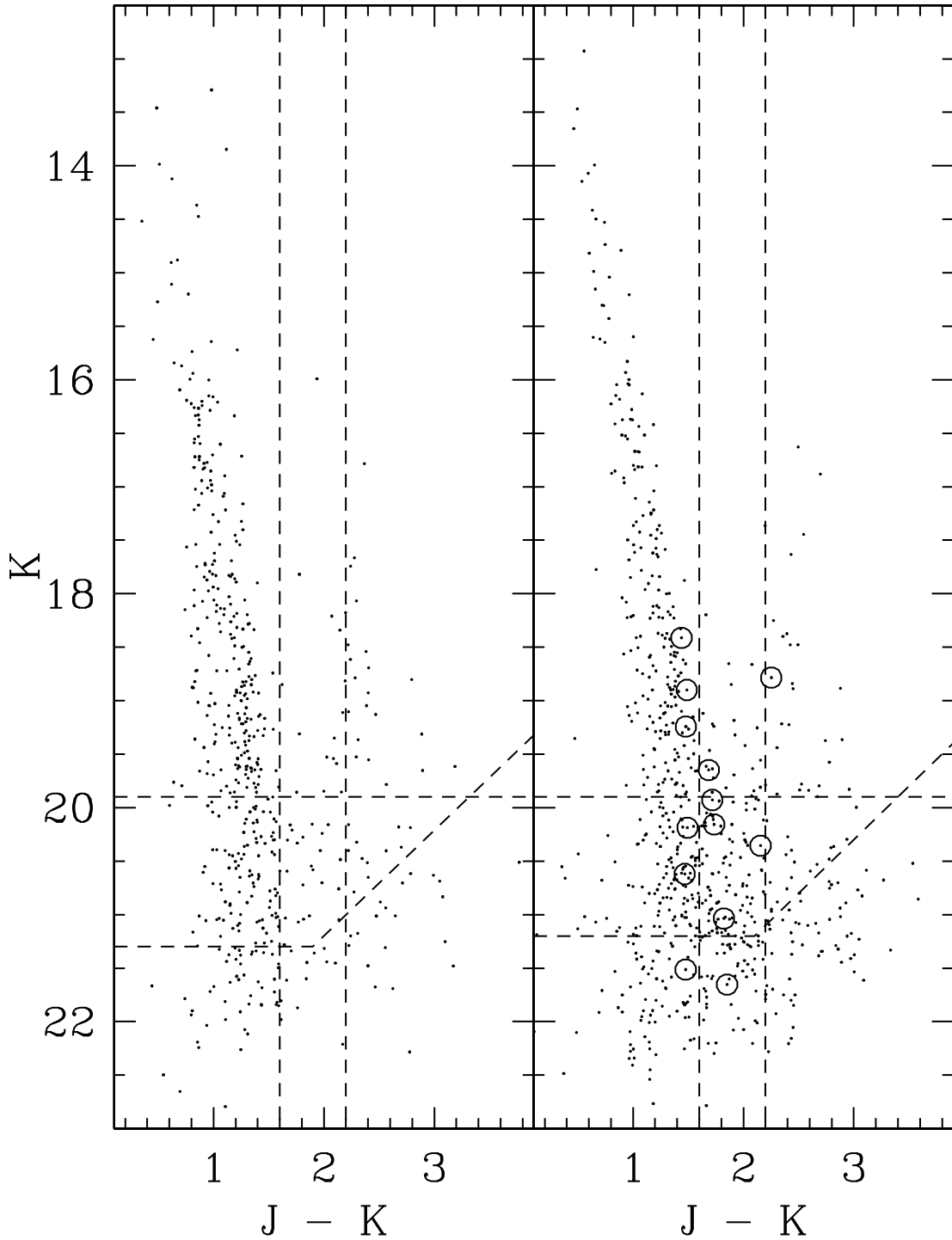
FIG. 6.—CMDs for reference ( left ) and HIZSS 3 ( right ) fields. Only stars with \sigma_{J-K} \leq 0.5 mag are shown. The HIZSS 3 TRGB edge at K = 19.90 \pm 0.09 is indicated by a horizontal dashed line. The combination of the J and K completeness limits are shown as connected dashed horizontal and diagonal lines. The vertical dashed lines indicate the color region that contains the RGB candidates in the HIZSS 3 field. The circled objects in the HIZSS 3 ( right ) panel indicate stars that are spatially coincident with the H II region emission-line gas. See text for more details.
