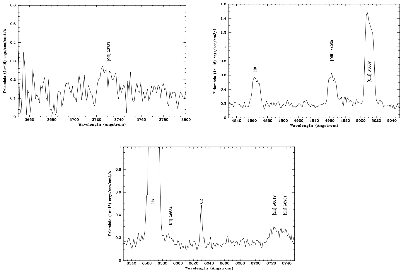
FIG. 1.—Three spectral regions in our summed spectrum of the H II region in HIZSS 3.
