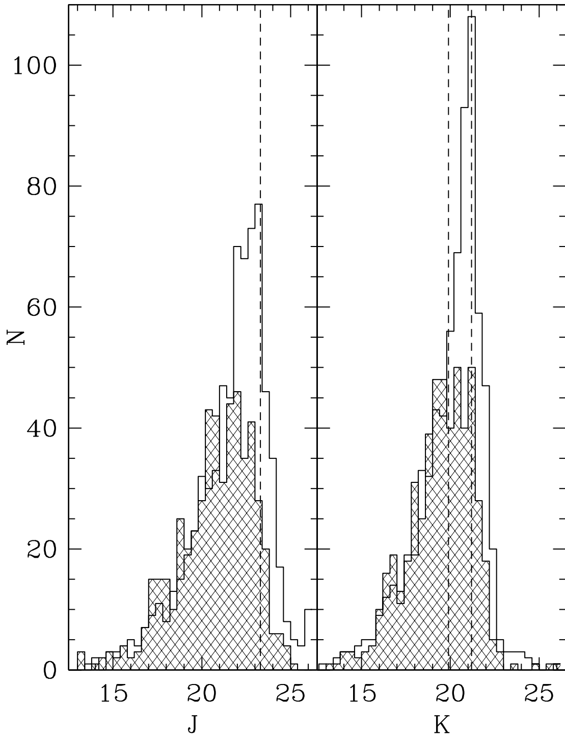
FIG. 4.— J and K luminosity functions for the stellar objects in the HIZSS 3 and reference field images with J and K magnitudes. The bin size is 0.4 mag. The hatched luminosity functions contain the 525 stellar objects in the reference field. The nonhatched luminosity functions contain the 727 stellar objects in the HIZSS 3 field. The vertical dashed line in the J panel indicates the completeness limit in the HIZSS 3 field. The vertical dashed lines in the K panel indicate the adopted TRGB apparent magnitude and the completeness limit in the HIZSS 3 field. [See the electronic edition of the Journal for a color version of this figure.]
