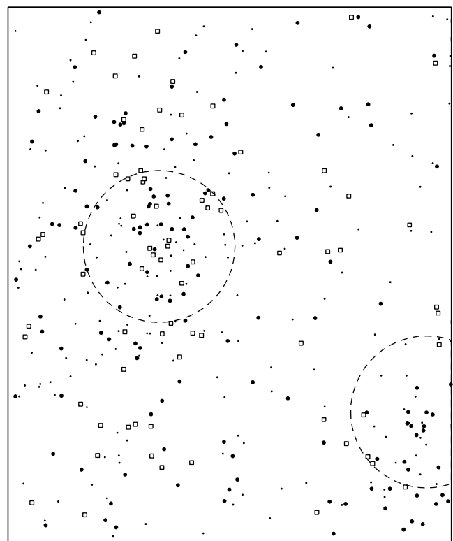
FIG. 8.—Distribution of objects in HIZSS 3 field grouped by color. North is up, east is to the left, and the field of view is 2.35 \times 2.35 in size (cf. HIZSS 3 K_s image in Fig. 2). Only objects with K \geq 19.9 and \sigma_{J-K} \leq 0.5 are shown. Small filled circles correspond to J - K < 1.6 . Large filled circles correspond to 1.6 \leq J - K \leq 2.2 (i.e., the HIZSS 3 red giant candidates). Open squares correspond to J - K > 2.2 . The upper dashed circle is centered on the VLA H I peak, while the lower dashed circle is centered on the H II region. Circle centers correspond to coordinates published by MHK03. The circle radii are 20'' . [See the electronic edition of the Journal for a color version of this figure.]
