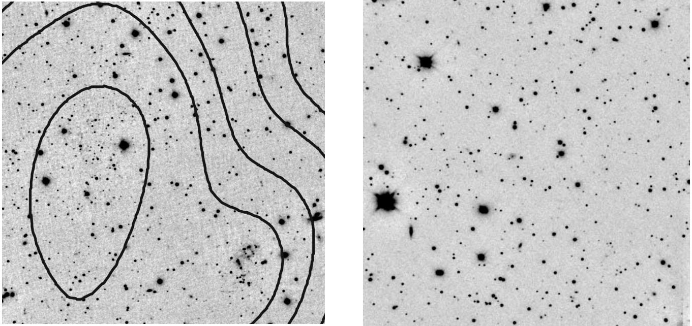
FIG. 2.— K_s HIZSS 3 ( left ) and reference field ( right ) images. North is up, and east is to the left. Each image is 2'.35 \times 2'.35 in size. In the HIZSS 3 image, the H I contours from MHK03 are overlaid (see their Fig. 1). From inspection, it is clear that there is a faint stellar population associated with the H I peak, while the H II region lies within a bulge in the H I contours. Objects in the reference field are more uniformly distributed and less numerous.
