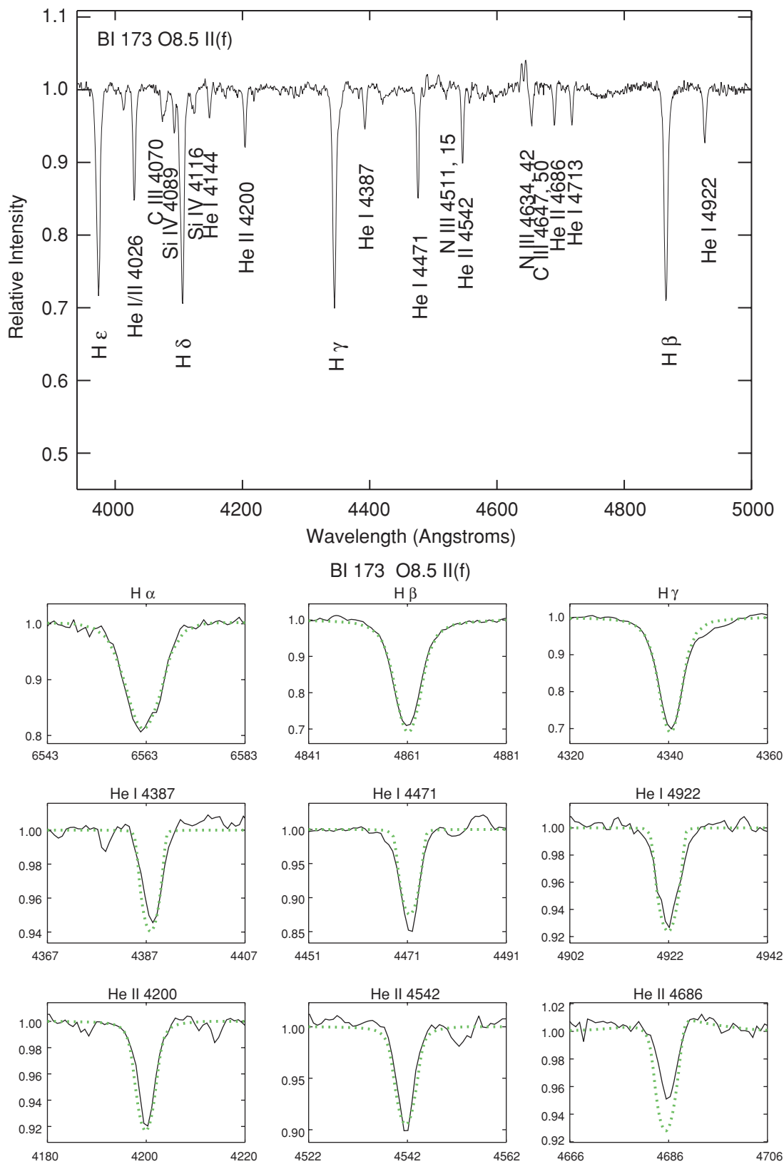
Figure 22. BI 173. The upper figure shows a section of the blue spectrum of this star, with the prominent lines identified. The lower figure shows the fits (dotted) for the principal diagnostic lines.
