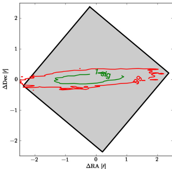
Figure 9. 1\sigma (green) and 99% (red) uncertainty in the position of a particular object ( 120^\circ solar elongation), 30 days after discovery. The field of view of ACS/WFC is overlaid as a black square.
