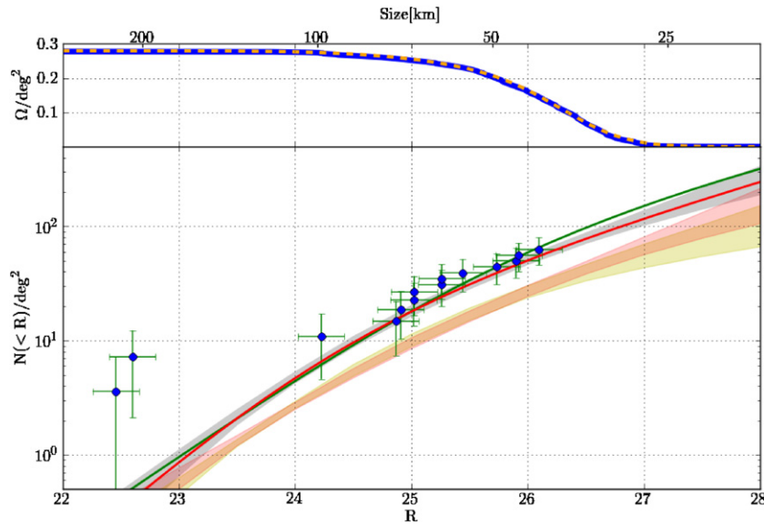
Figure 4. Top panel shows the effective area surveyed in this paper as a function of R magnitude in blue. While that function depends on the efficiency function and shared area of every pointing in this survey, we can simplify the \sim 2000 parameters (see Equation (3)) into the four parameters of the function plot in dashed orange (see Equation (5)). The lower panel shows the luminosity function of objects found in this survey, normalized by the effective area at each magnitude. The best model in Fuentes et al. (2009) is overplotted in green, while the best model for all surveys, including this one, is shown in red. The gray area represents the area enclosed by the 1\sigma confidence region for all surveys. The lower set of shaded areas represents the 1\sigma confidence limits for the cumulative function of the hot (red) and cold (yellow) populations.
