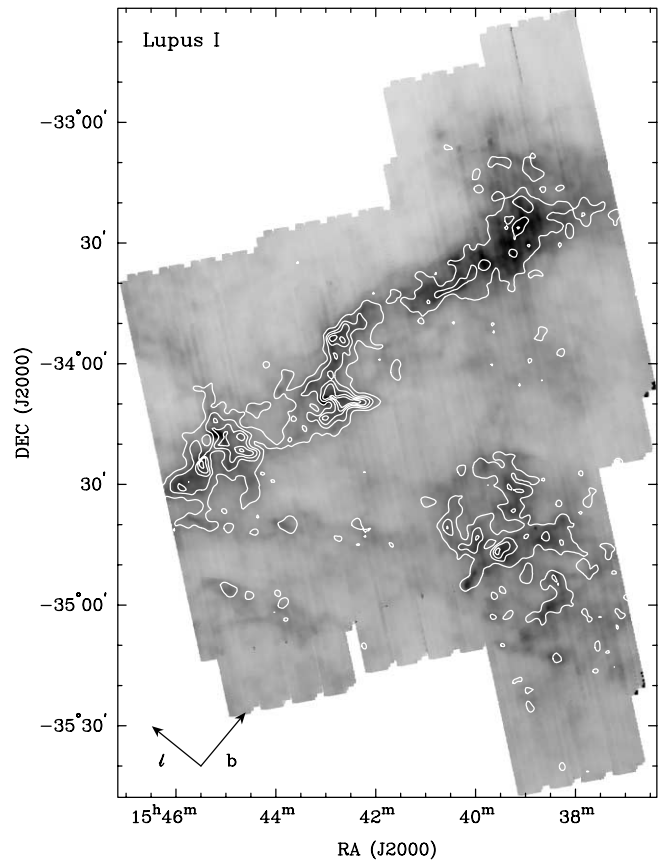
FIG. 14.—Magnitudes of visual extinction (contours) are overlaid on the 160\ \mu\text{m} emission map for Lupus I. The contours range from 3 to 15 A_V , in steps of 3 A_V . The extinction map has 2' resolution. We have also shown the direction of increasing Galactic l and b coordinates.
