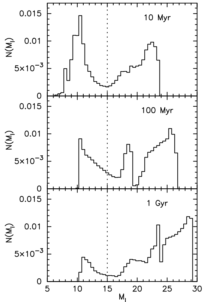
FIG. 8.—Model I -band cluster luminosity functions for \alpha_2 = 1.0 and ages 10, 100, and 1000 Myr, with the I -band sensitivity limit (dotted line) from Bouvier et al. (1998). This limit corresponds to 90% completeness in 1200 s using the University of Hawaii 8 K CCD mosaic at the CFHT for a cluster at 200 pc. Note that this sensitivity limit lies in the middle of the stellar/substellar trough for each of the model clusters. This implies that most ground-based I -band searches are unable to detect peak D, except in relatively young nearby clusters.
