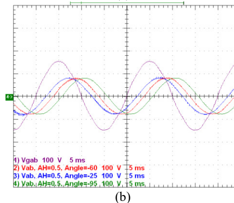
Fig. 18. Comparison of voltage synthesis ability for the hexagonal chopper: (a) constant duty cycle; (b) heterodyne method.
