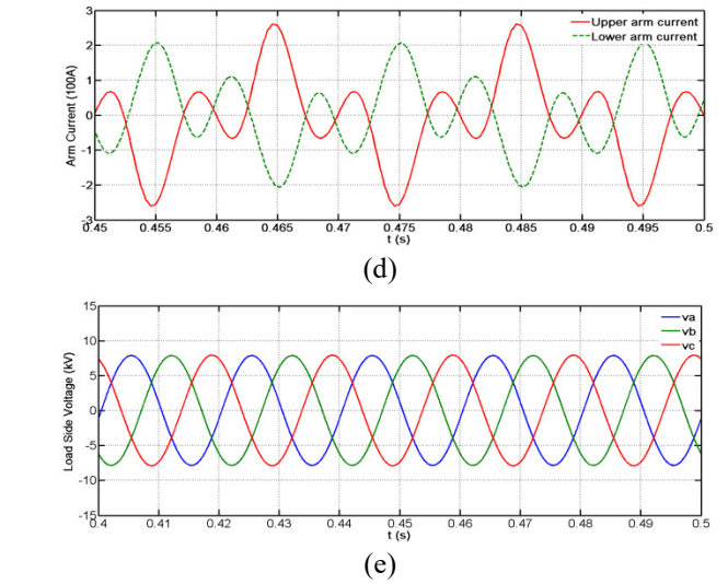
Fig. 12. Simulation results: (a).chopped output voltage for one phase; (b).quasi-2-level mode with 5-step voltage transition and output/arm currents; (c).voltage balancing results; (d).upper and lower arm currents after moving average filter; (e).three-phase output voltage.
