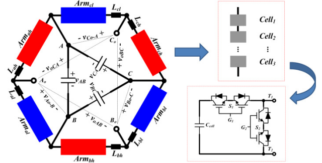
Fig. 3. Proposed M2AHC with its arm and cell structures.
