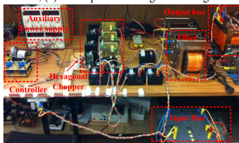
Fig. 17. Photo of the experiment setup for hexagonal chopper system.
