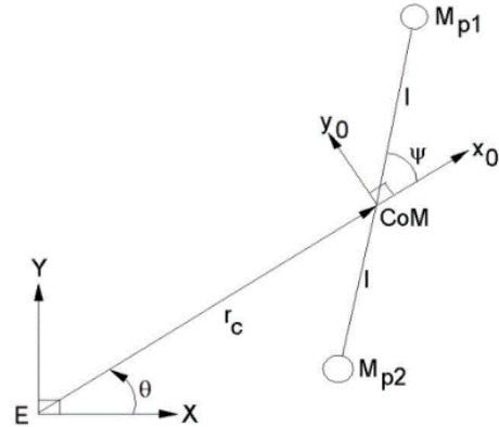
Fig. 21. Planar tether system
