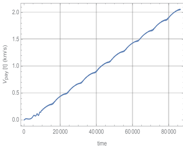
Fig. 5. Tangential velocity of the sub-spans relative to the spin axis with time.
