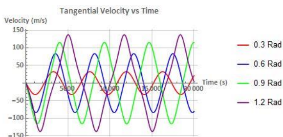
Fig. 24. An example of the tangential velocity vs time chart for a tether system.
