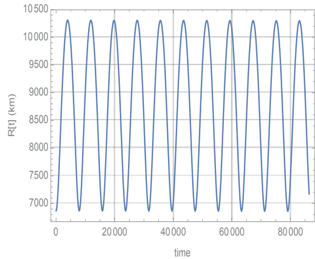
Fig. 7. Magnitude of position vector R with time.
