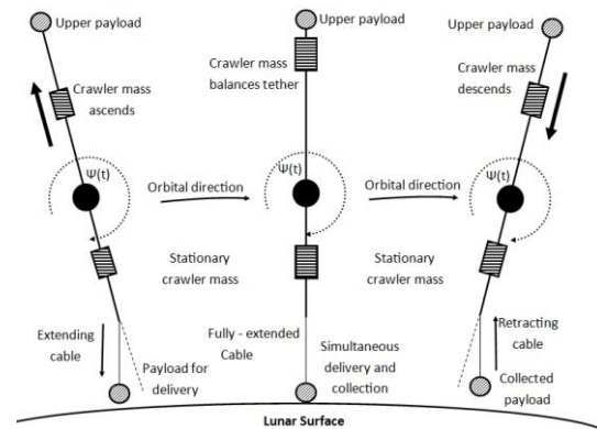
Fig. 17. Proposed lunavator design and payload transfer method
