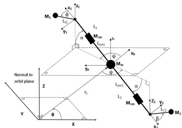
Fig. 18. 3D schematic representation of proposed lunavator
