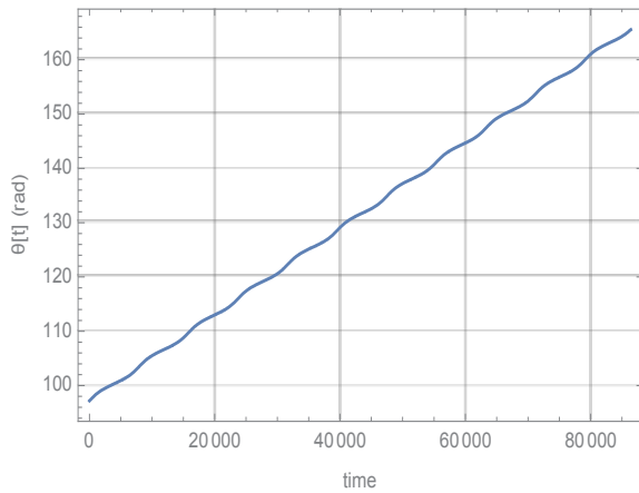
Fig. 9. True anomaly with time.
