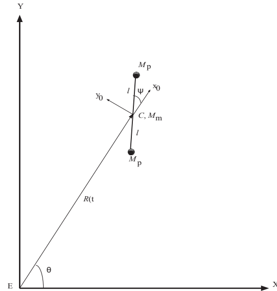
Fig. 2. A planar dumb-bell tether in LEO where E represents the centre of the Earth and EXY is an Earth fixed frame.
