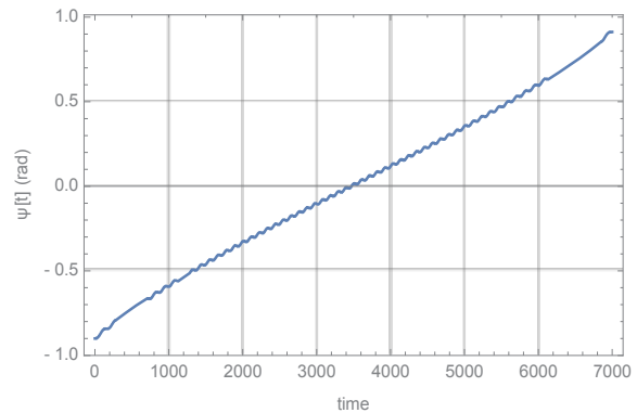
Fig. 15. Spin-up of tether on a circular orbit, with activated axial position restoration force as well as motor torque.
