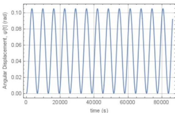
Fig. 20. In-plane libration of 580km tether with 2,000kg payloads, 1,000 tonne motor mass, 145 MNm torque
