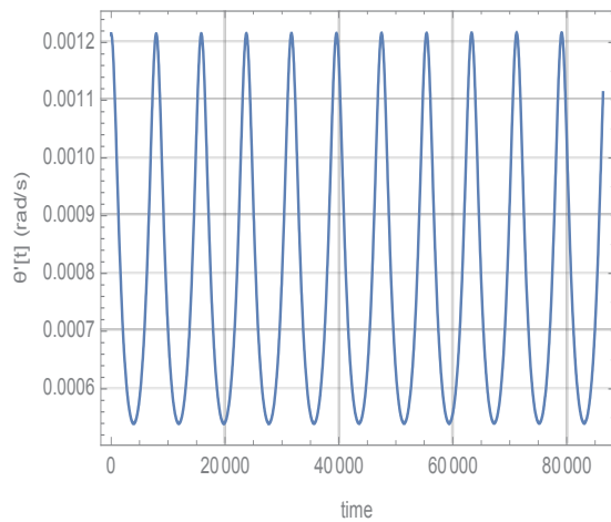
Fig. 10. Rate of change of true anomaly with time.
