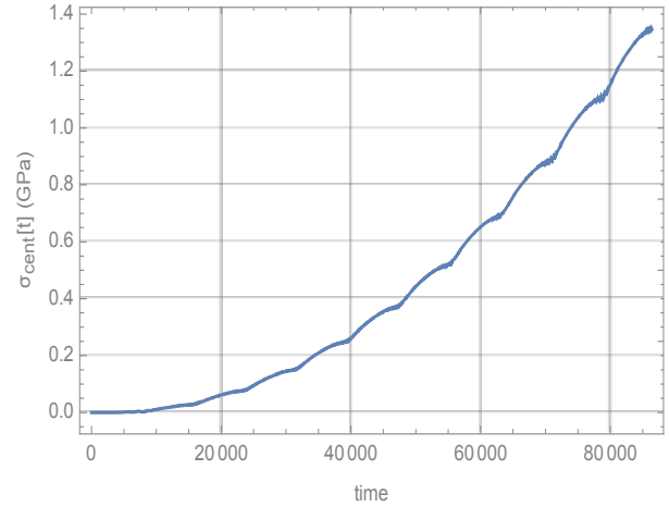
Fig. 6. Sub-span centripetal stress with time.
