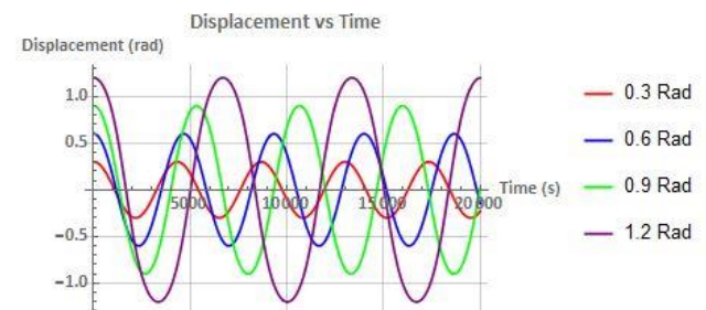
Fig. 22. An example of the angular displacement vs time chart for a tether system.
