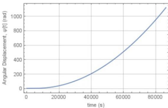
Fig. 19. Continuous spin of 580km tether with 2,000kg payloads, 1,000 tonne motor mass, 1000 MNm torque
