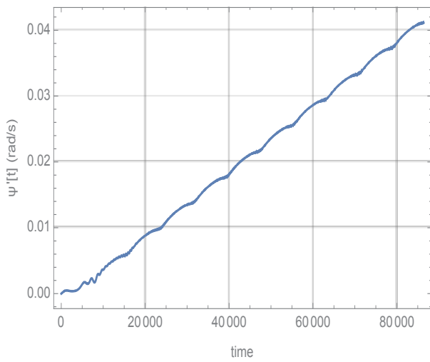
Fig. 4. Angular rate of the tether with time.
