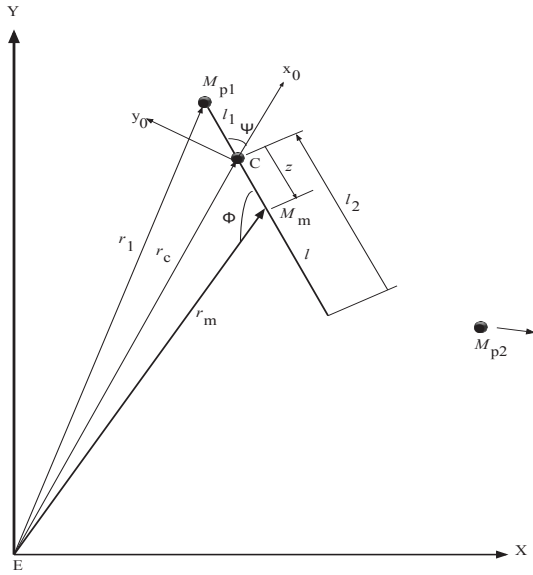
Fig. 13. Asymmetrical tether in the Earth-fixed frame with asymmetry due to the unplanned loss of payload M_{p2} .
