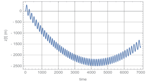
Fig. 14. Effect of axial propulsive force of 5.5kN on z(t) with time.
