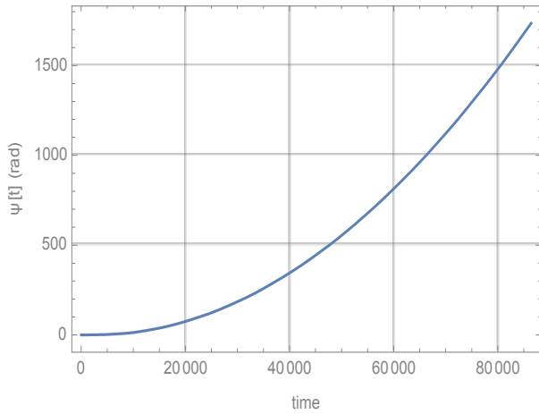
Fig. 3. Angular displacement of the tether with time.
