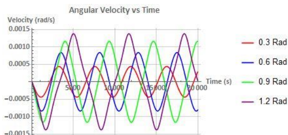
Fig. 23. An example of the angular velocity vs time chart for a tether system
