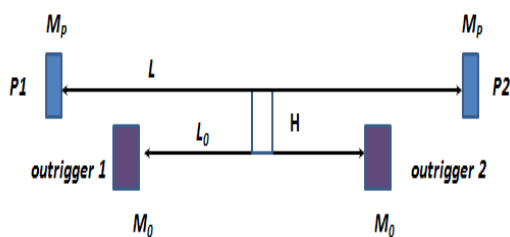
Fig. 11. Side elevation of the tether showing the propulsion and outrigger tethers and the separation distance H between them.
