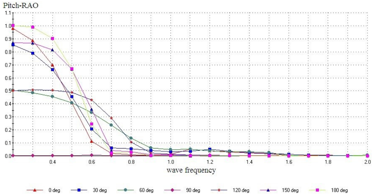
Fig. 2. Pitch RAO for 22 knots in regular waves
