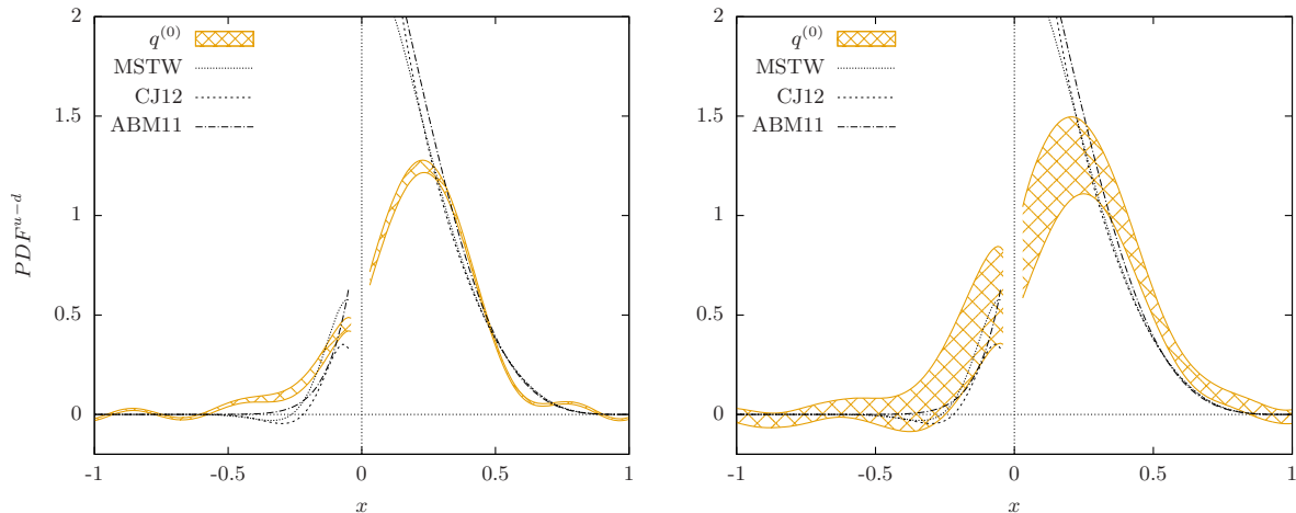
Figure 6: Results from an hypothetical mixed momentum analysis using different values of the momentum in the computation of the lattice matrix element ( left: P_3 = 4\pi/L , right: P_3 = 6\pi/L ) than in the Fourier transformation, matching and mass corrections ( P_3 = 8\pi/L ) with 5 steps of HYP smearing.
