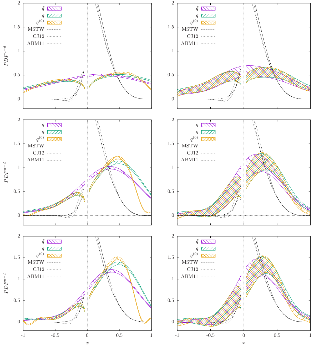
Figure 5: The resulting quasisdistribution \tilde{q} , PDF without subtracting the mass correction q , and final PDF q^{(0)} , left: P_3 = 4\pi/L , right: P_3 = 6\pi/L , from top to bottom: 0 steps, 2 steps, 5 steps of HYP smearing, negative region: \tilde{q}(x) = -q(-x) , comparison with phenomenological u(x) - d(x) curves at Q^2 = 6.25 \text{ MeV}^2 (MSTW [29], CJ12 [30], ABM11 [31]).
