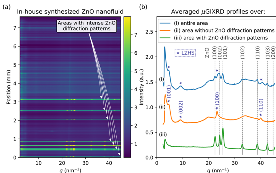
Figure 7. \mu GIXRD analysis of the residual surface patterns from evaporative drying of a 30 \mu\text{L} ZnO nanofluid sessile droplet on an \sim 1 \times 1 \text{ cm}^2 silicon wafer at room temperature and relative humidity of \sim 45\% . The nanofluid was prepared from the in-house synthesized ZnO nanoparticles, dispersed in a mixture of cyclohexane and isobutylamine (5:1 volume:volume ratio). (a) shows a 2D intensity heat map with respect to position of the scan point on the sample (along z -axis in Figure 1) and momentum transfer vector, q . Arrows show regions of the sample that produced intense ZnO diffraction patterns. Intensity (a.u.) shown in (a) was calculated as a percentile in the range 0.05–99.95% for better contrast. (b) \mu GIXRD line profiles averaged over (i) the entire scan area, (ii) the area that did not show ZnO diffraction patterns, and (iii) the area with intense ZnO diffraction patterns, marked with arrows in (a). ZnO peaks are indexed in accordance with the reference pattern (PDF 01-075-0576), and layered zinc hydroxide (LZH) structures are labeled with star markers “★” and indexed according to refs 44 and 45.
