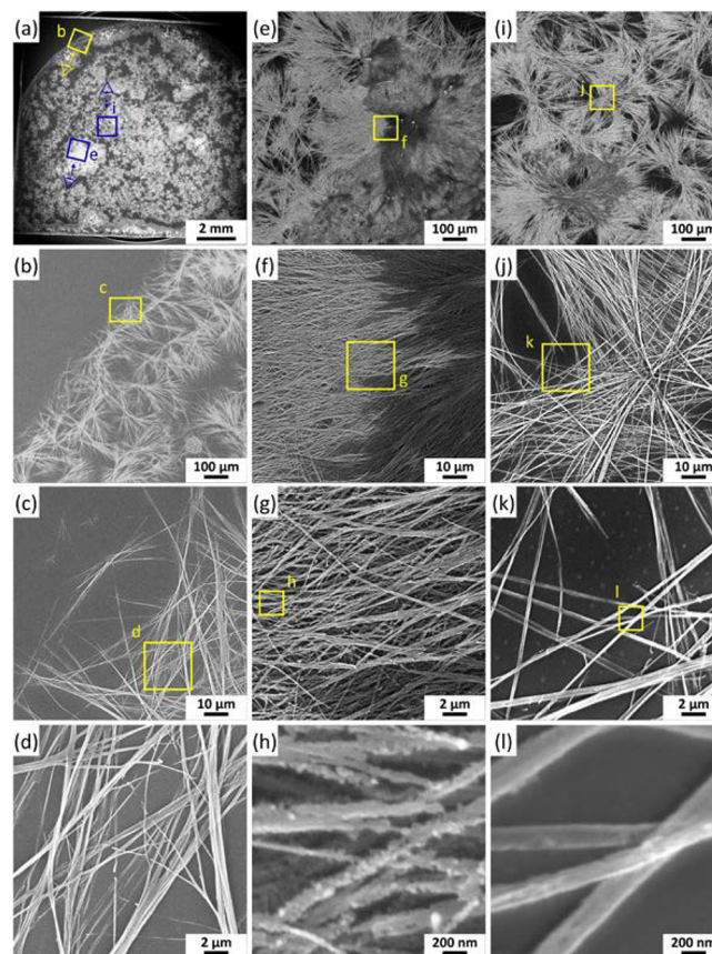
Figure 4. SEM images of the residual surface patterns from evaporative drying of a 30 \mu\text{L} ZnO nanofluid sessile droplet on an \sim 1 \times 1 \text{cm}^2 silicon wafer at room temperature and relative humidity of \sim 45\% . The nanofluid was prepared from the in-house synthesized ZnO nanoparticles, dispersed in a mixture of cyclohexane and isobutylamine (5:1 volume:volume ratio). The rectangular regions in the figures are enlarged, with their labels corresponding to those of the figures. The schematic drawings of the eye and arrow in (a) indicate the direction of viewing of the regions as shown in their corresponding magnified images.
