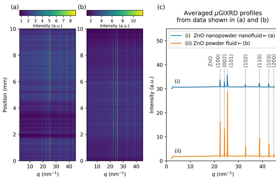
Figure 8. \mu GIXRD analysis of the residual surface patterns from evaporative drying of a 30 \mu\text{L} ZnO (nano)fluid sessile droplets on a \sim 1 \times 1 \text{ cm}^2 silicon wafer at room temperature and relative humidity of \sim 45\% . The (nano)fluids were prepared from commercially acquired ZnO nanopowder and ZnO powder, dispersed in a mixture of cyclohexane and isobutylamine (5:1 volume:volume ratio). (a) and (b) show 2D intensity heat maps for surface patterns from ZnO nanopowder and ZnO powder (nano)fluids, respectively. These heat maps are plotted with respect to position of the scan point on the sample (along the z -axis in Figure 1) and momentum transfer vector, q . Intensities (a.u.) in (a) and (b) were calculated as a percentile in the range 0.1–99.9% and 0.3–99.7%, respectively, to improve the contrast. (c) \mu GIXRD line profiles averaged over the entire scan areas for (i) patterns from ZnO nanopowder nanofluid (data in (a)) and (ii) patterns from ZnO powder fluid (data in (b)).
