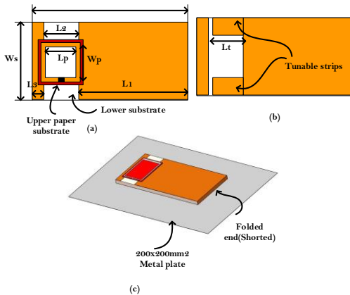
Fig. 2. Dimensions (mm) of Proposed tag antenna (a) RFID tag (b) RFID tag with tuning strip (c) RFID tag on metal plate ( L_s=50, W_s=25, L_1=38.5, L_2=8.5, L_3=, L_p=18, W_p=12, L_t=8 )
