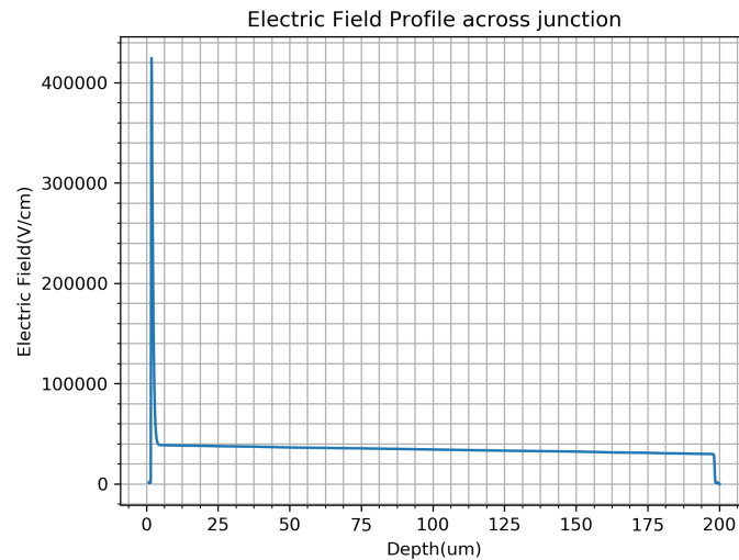
Figure 3. Typical electric field profile through device showing high electric field at junction between n+/p region. The device is 200 \mu\text{m} thick with a reverse bias of 700 V.
