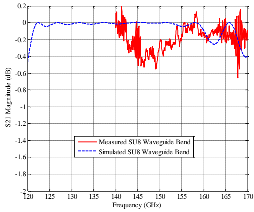
Fig. 10. S_{21} Results of 150 GHz waveguide
