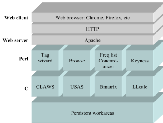
Figure 1: Wmatrix architecture.
