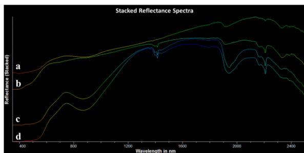
Figure 2. Stacked VISNIR reflectance spectroscopy data from each of the four zones of the dike. Moving from top to bottom, these zones include the ‘fresh’ zone (a), the ‘green’ zone (b), the ‘purple’ zone (c), and the ‘red’ zone (d).
