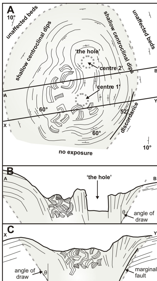
Fig. 12 Field sketches of structure number 3. a Plan view; b, c Cross sections along lines shown in a . Angle of draw ( \theta ) is the angle at which the subsidence spreads out; it defines the limit for subsidence effects (Whittaker and Reddish 1989; Ren and Li 2008). In a , ‘centre 1’ and ‘centre 2’ refer to the locations of two possible buried ice blocks whose mutual melting caused the subsidence structure to have an elongated, ‘figure of eight’ configuration (see text for details). Note the presence of breccia sandwiched between tilted beds in b , suggesting that subsidence was probably sequential (piecemeal)
