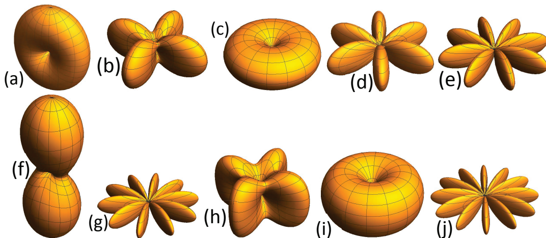
Figure 8. (colour online) Angular distribution of the predicted power distribution from the excitation of each of the ten lowest frequency EM cavity modes of an imperfect disk BSCCO device. (a)(1,1); (b) (2,1); (c) (0,1); (d) (3,1); (e) (4,1); (f) (1,2); (g) (5,1); (h) (2,2); (i) (0,2); (j) (6,1).
