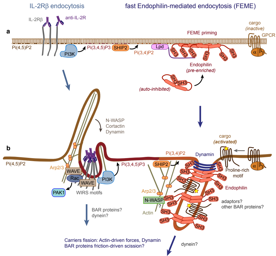
Figure 1. Cargo capture and local membrane bending by cytosolic proteins
