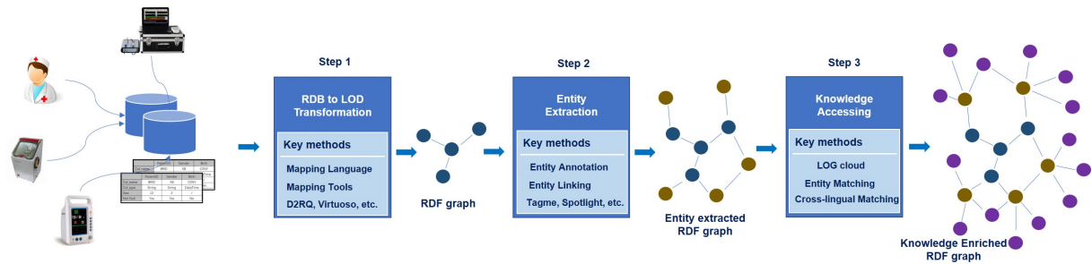
FIGURE 1. The pipeline of the method. The input of the method is various data records from IoT devices, doctors, HIS records, etc. The output of the method are the enriched HIS records with medical knowledges from LOD. The module “RDB to LOD Transformation” is introduced in section III-A-1. “Entity Extraction” is described in section III-A-2. “Knowledge Access” is proposed in section III-B.
