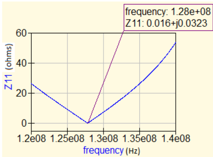
Figure 2.15 Input impedance as a function of frequency for port on rung
