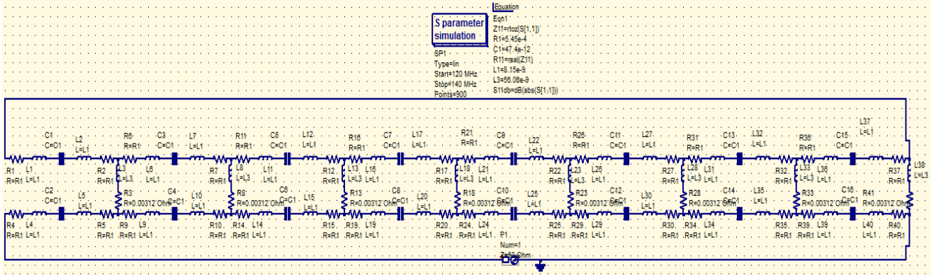
Figure 2.14 Schematic of a high-pass birdcage resonator designed in QUCS for port on a rung
