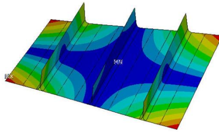
Figure 10. 90° degree surface ply orientation
