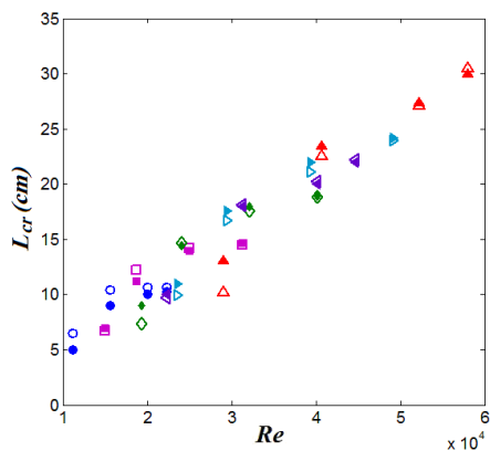
Fig.8. Comparison between the calculated and experimental values of L_{cr} . Symbols: experiments: ● D=5\text{cm} , ■ D=7\text{cm} , ◆ D=9\text{cm} , ◀ D=10\text{cm} , ▶ D=11\text{cm} , ▲ D=13\text{cm} for various incoming flow velocities; calculation using (8): the same symbols as experiments but open.
